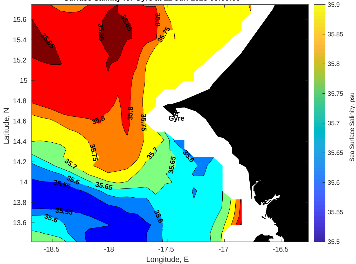
Surface Salinity for Gyre at 11-Jun-2025 00:00:00
