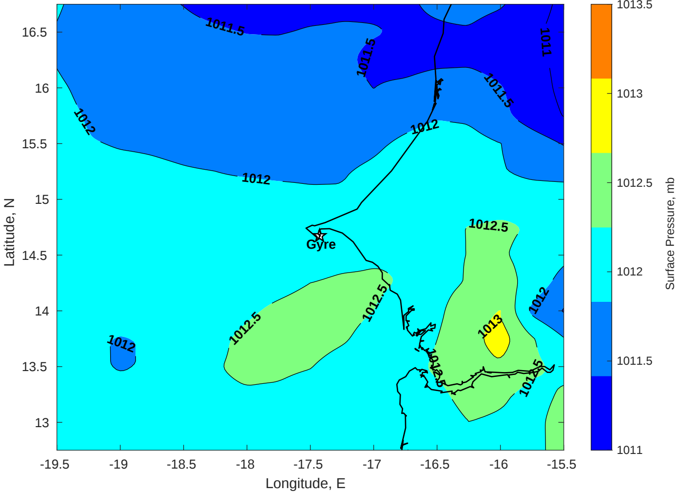
Surface Pressure (mb) for Gyre at 12-Jun-2025 00:00:00
