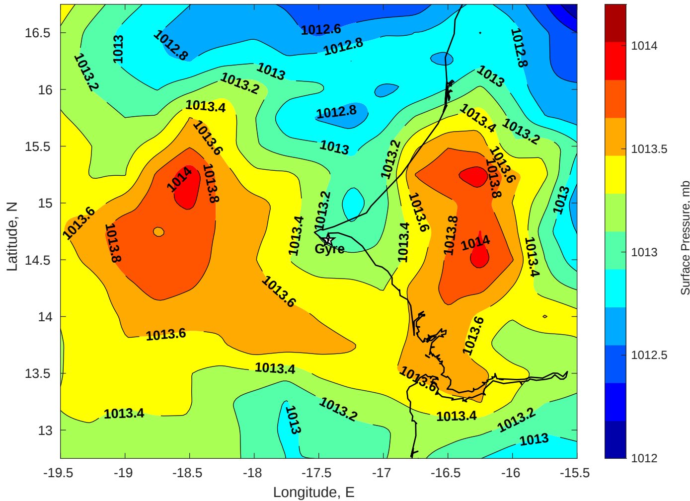
Surface Pressure (mb) for Gyre at 13-Jun-2025 00:00:00
