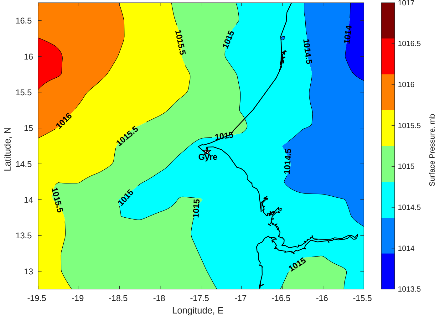
Surface Pressure (mb) for Gyre at 14-Jun-2025 00:00:00
