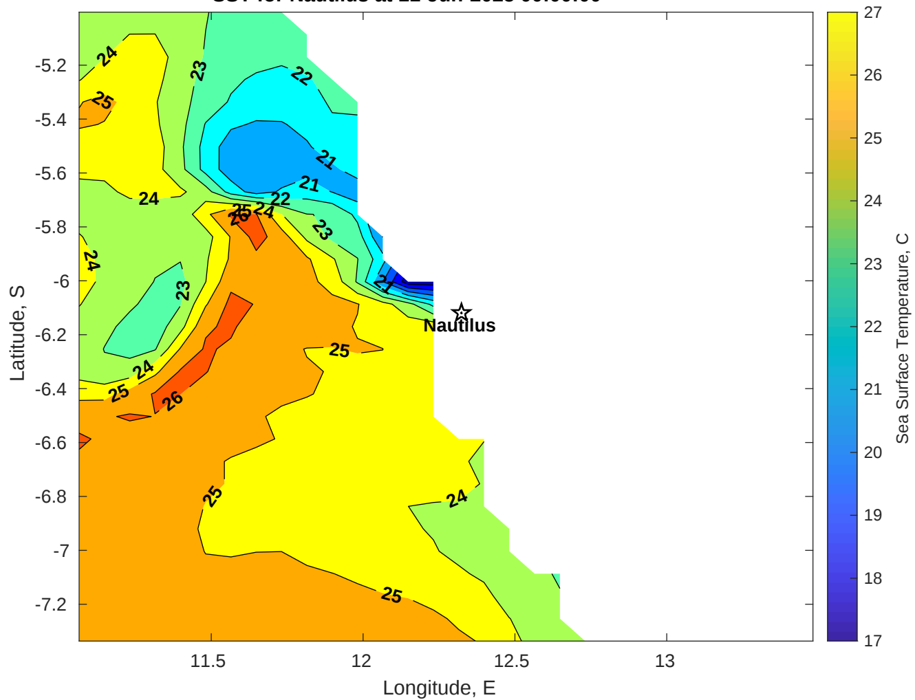
SST for Nautilus at 11-Jun-2025 00:00:00
