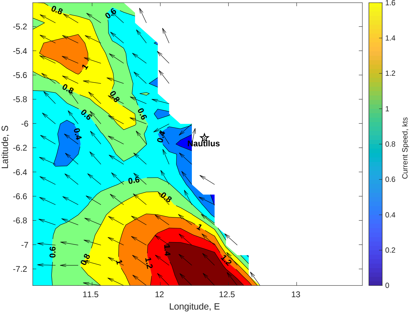
Surface Currents for Nautilus at 11-Jun-2025 00:00:00
