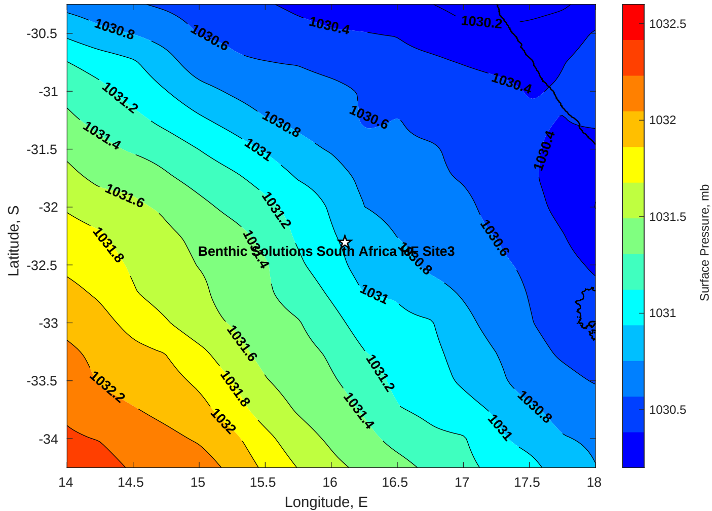
Surface Pressure (mb) for Benthic Solutions South Africa HF Site3 at 10-Jun-2025 00:00:00
