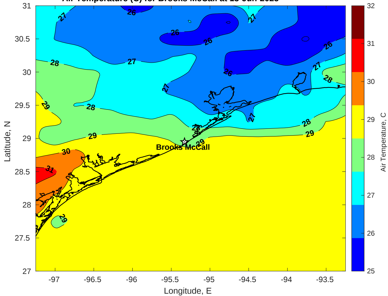
Air Temperature (C) for Brooks McCall at 13-Jun-2025
