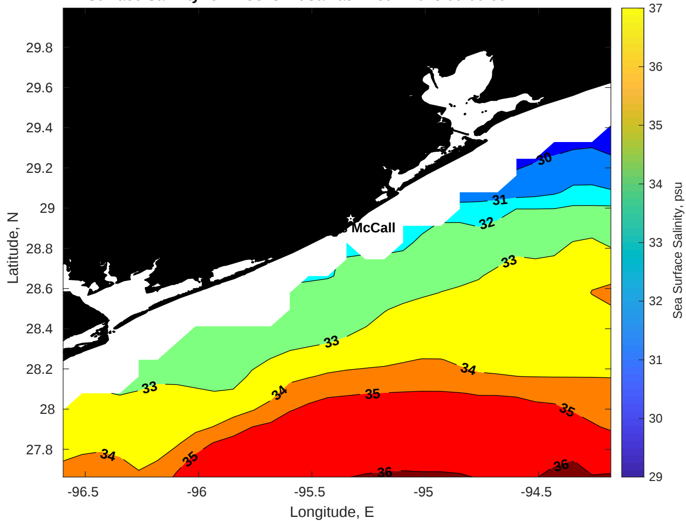
Surface Salinity for Brooks McCall at 12-Jun-2025 00:00:00
