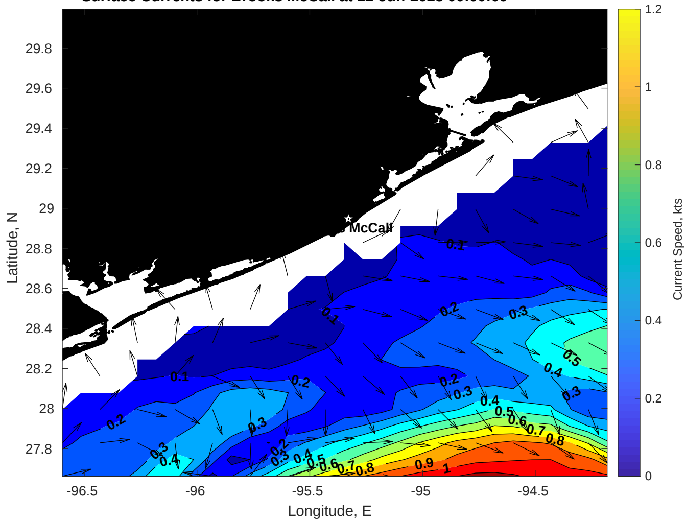
Surface Currents for Brooks McCall at 12-Jun-2025 00:00:00
