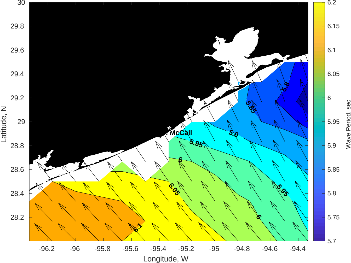
Wave Period (sec) for Brooks McCall at 13-Jun-2025 09:00:00
