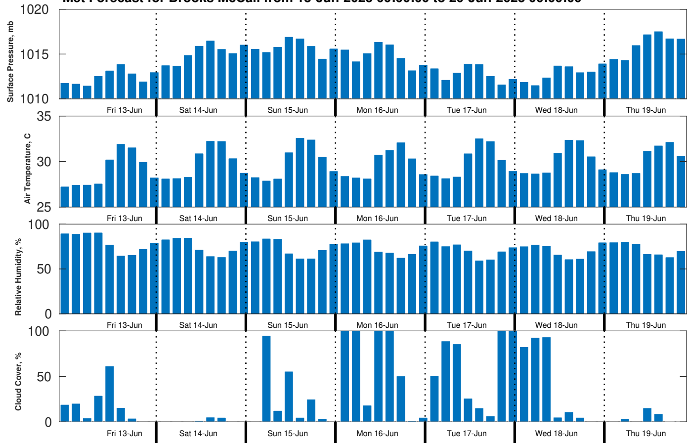
Met Forecast for Brooks McCall from 13-Jun-2025 00:00:00 to 20-Jun-2025 00:00:00
