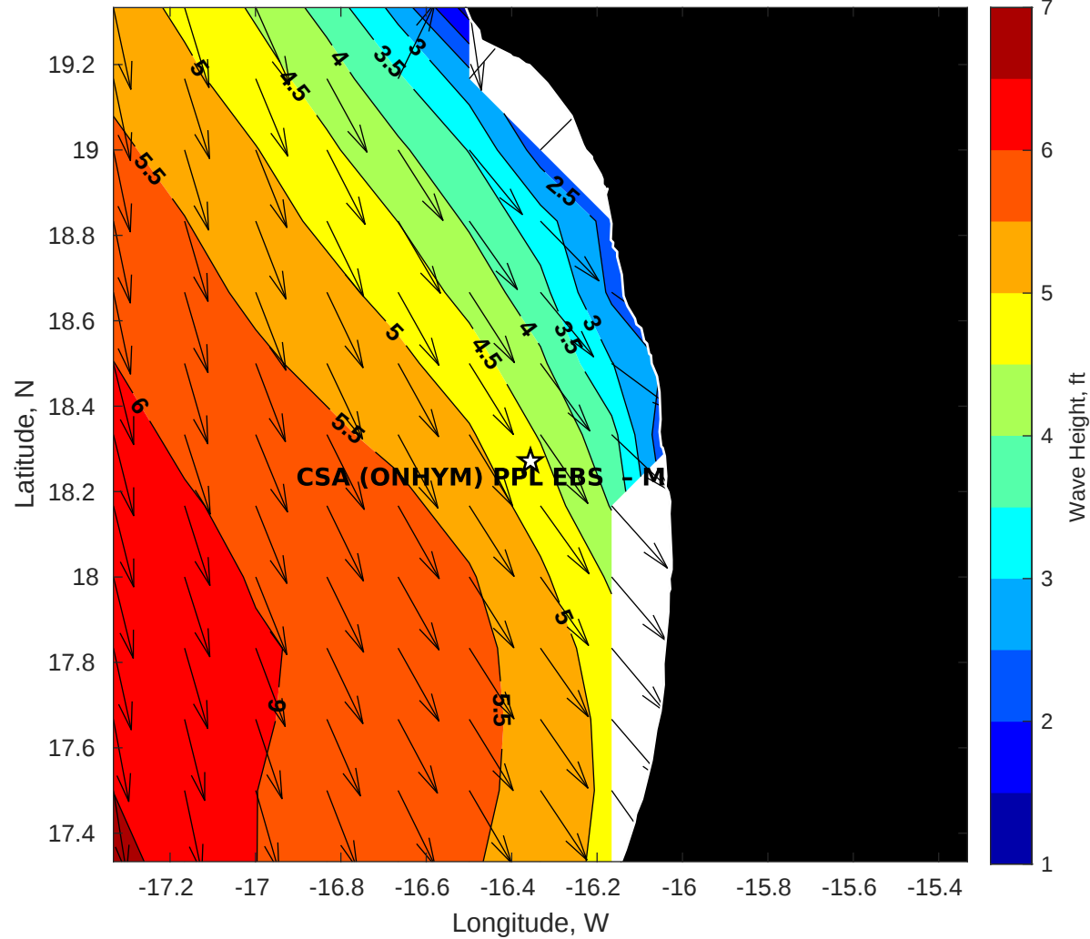
Wave Height (ft) for CSA (ONHYM) PPL EBS - Mauritania at 08-Jun-2025 09:00:00
