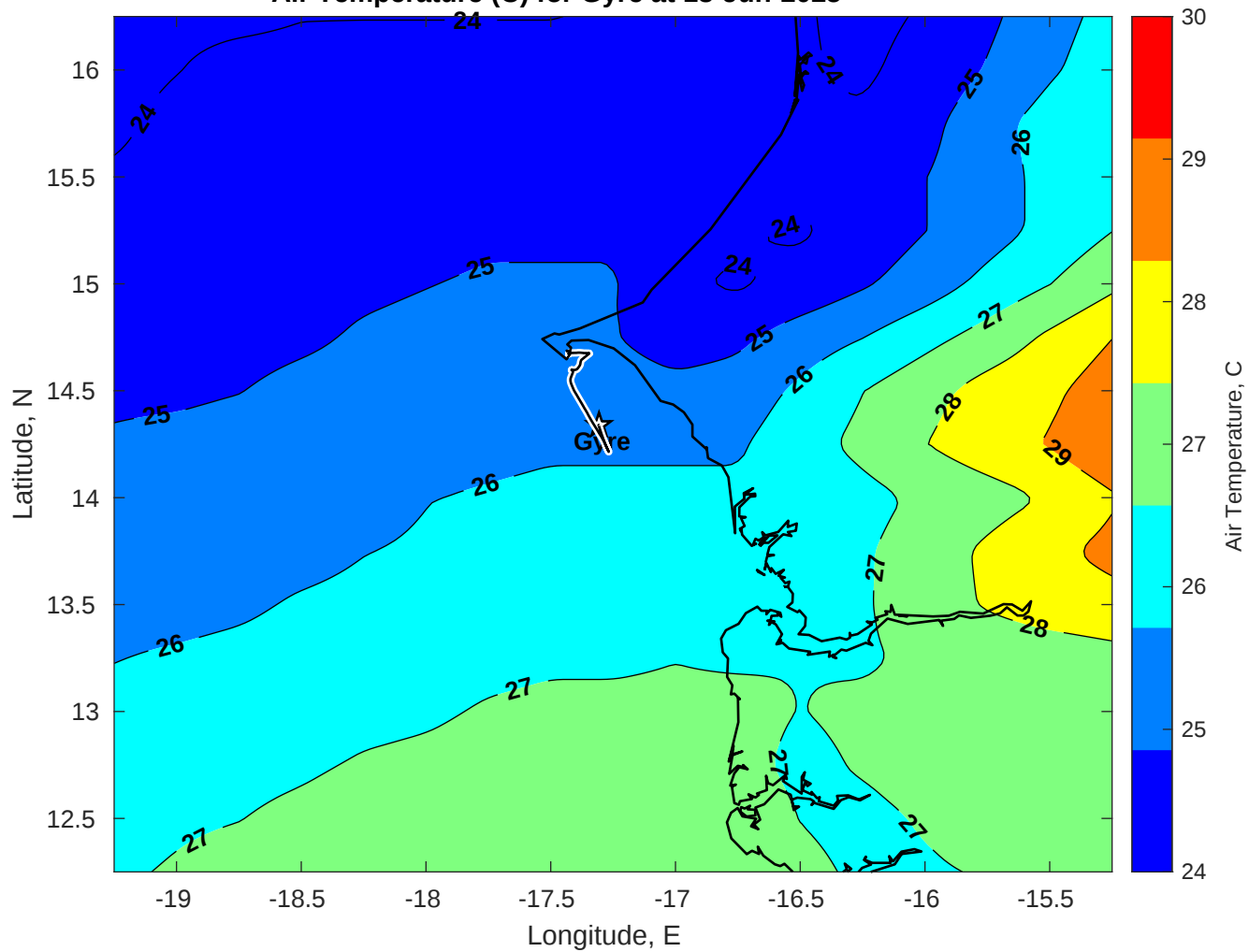
Air Temperature (C) for Gyre at 13-Jun-2025
