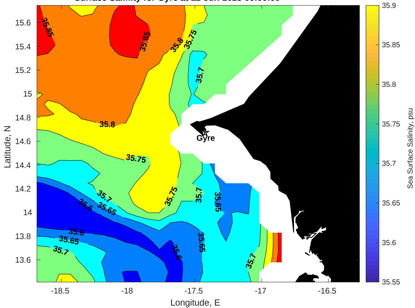
Surface Salinity for Gyre at 12-Jun-2025 00:00:00
