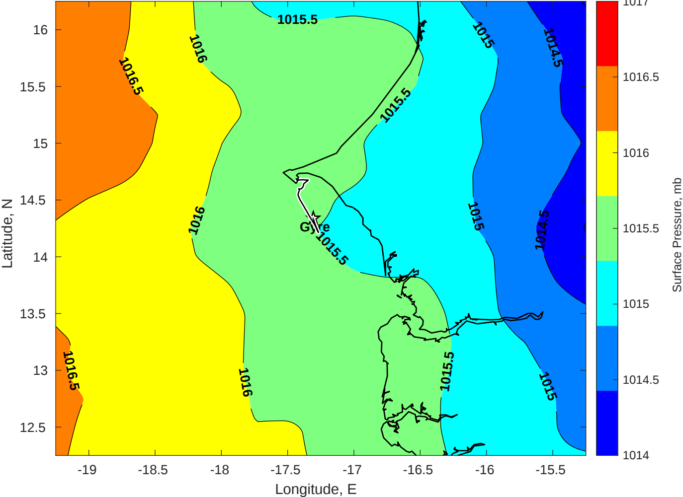
Surface Pressure (mb) for Gyre at 15-Jun-2025 00:00:00
