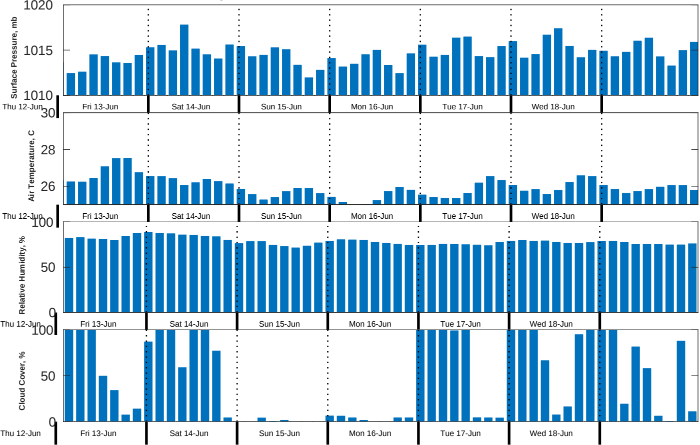
Met Forecast for Gyre from 12-Jun-2025 23:00:00 to 19-Jun-2025 23:00:00
