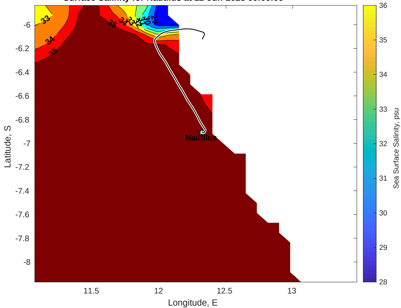
Surface Salinity for Nautilus at 12-Jun-2025 00:00:00
