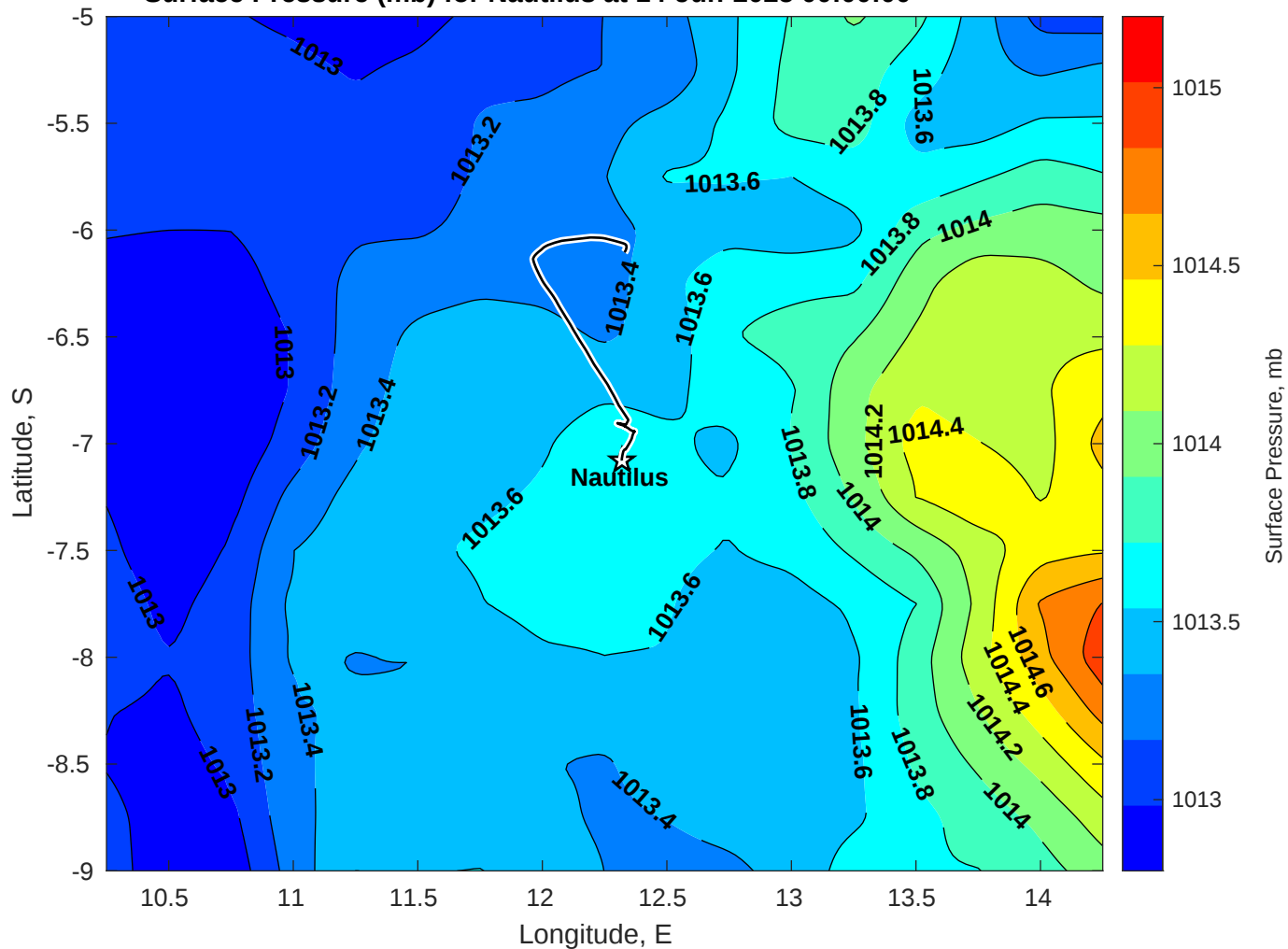
Surface Pressure (mb) for Nautilus at 14-Jun-2025 00:00:00
