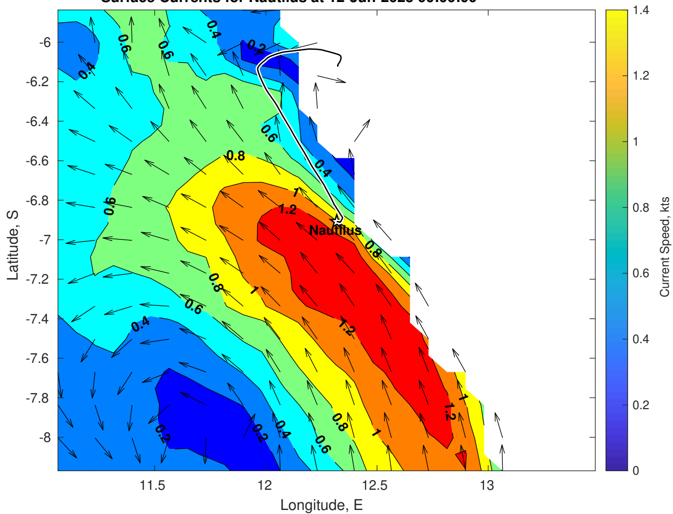
Surface Currents for Nautilus at 12-Jun-2025 00:00:00
