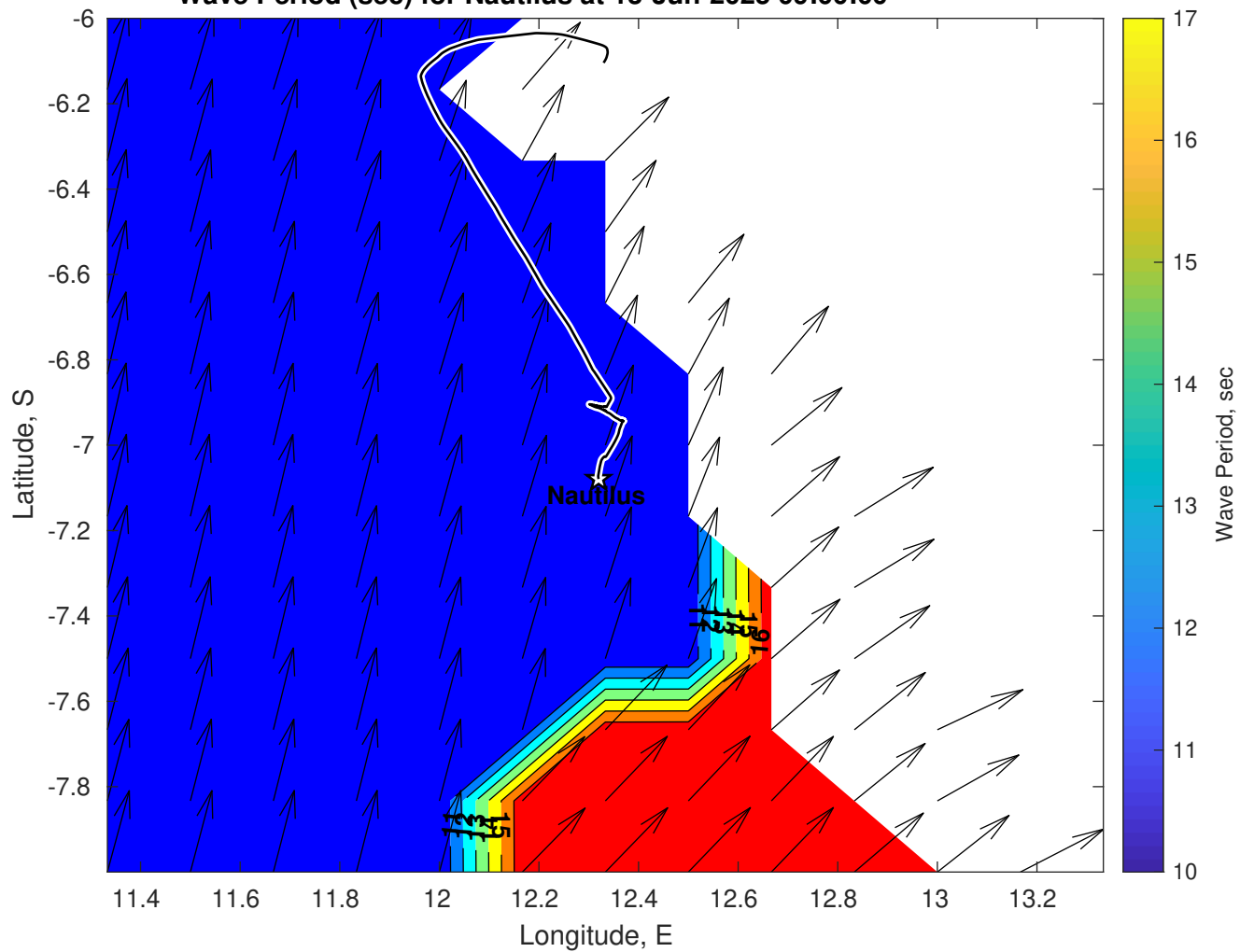
Wave Period (sec) for Nautilus at 13-Jun-2025 09:00:00
