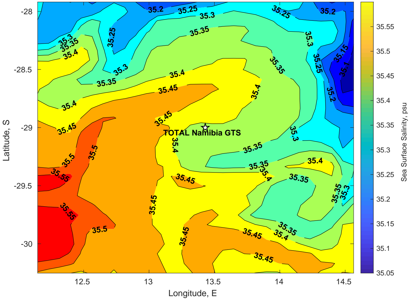
Surface Salinity for TOTAL Namibia GTS at 07-Jun-2025 00:00:00
