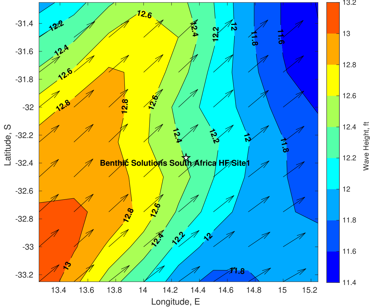
Wave Height (ft) for Benthic Solutions South Africa HF Site1 at 08-Jun-2025 09:00:00
