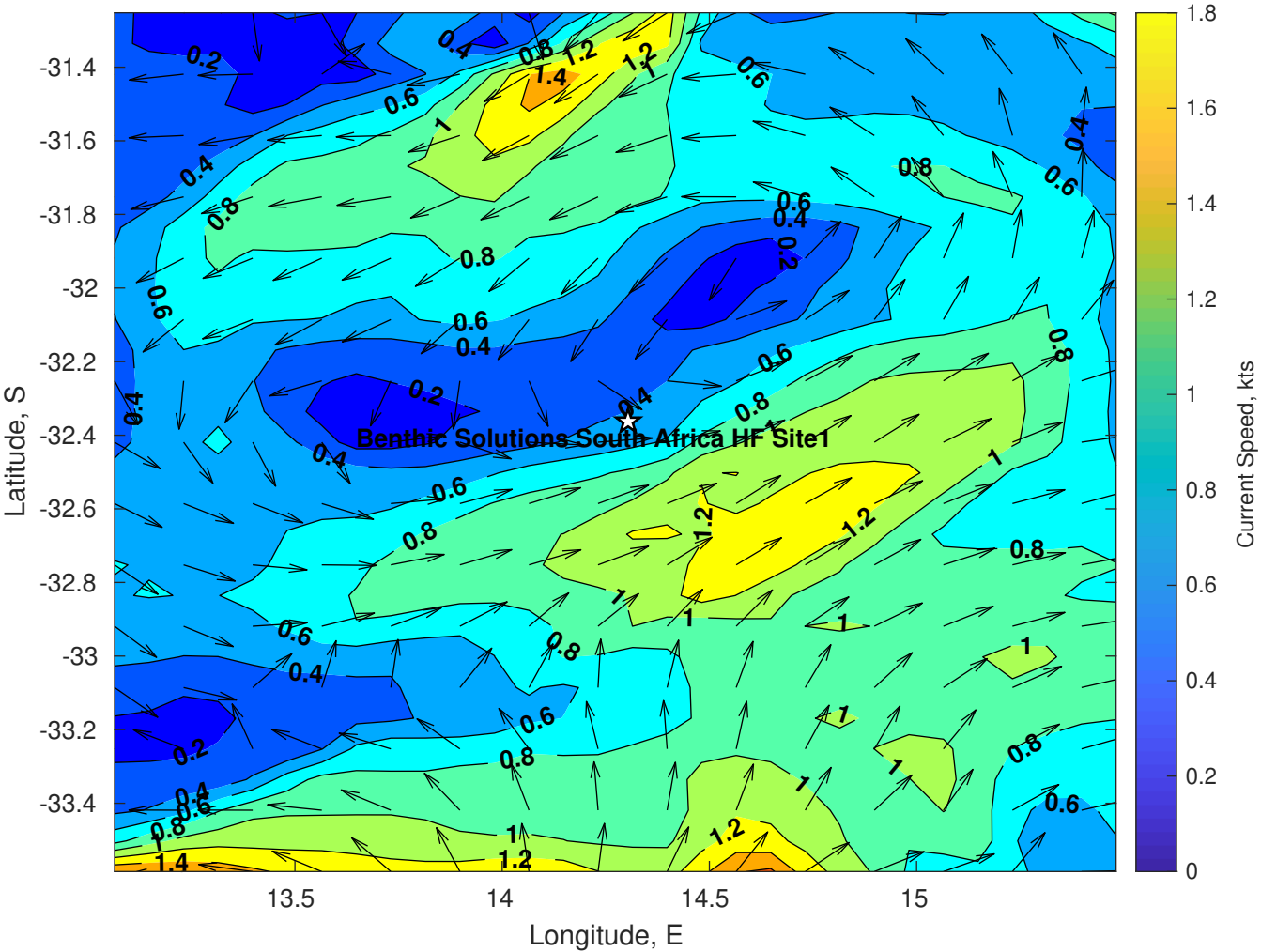
Surface Currents for Benthic Solutions South Africa HF Site1 at 07-Jun-2025 00:00:00
