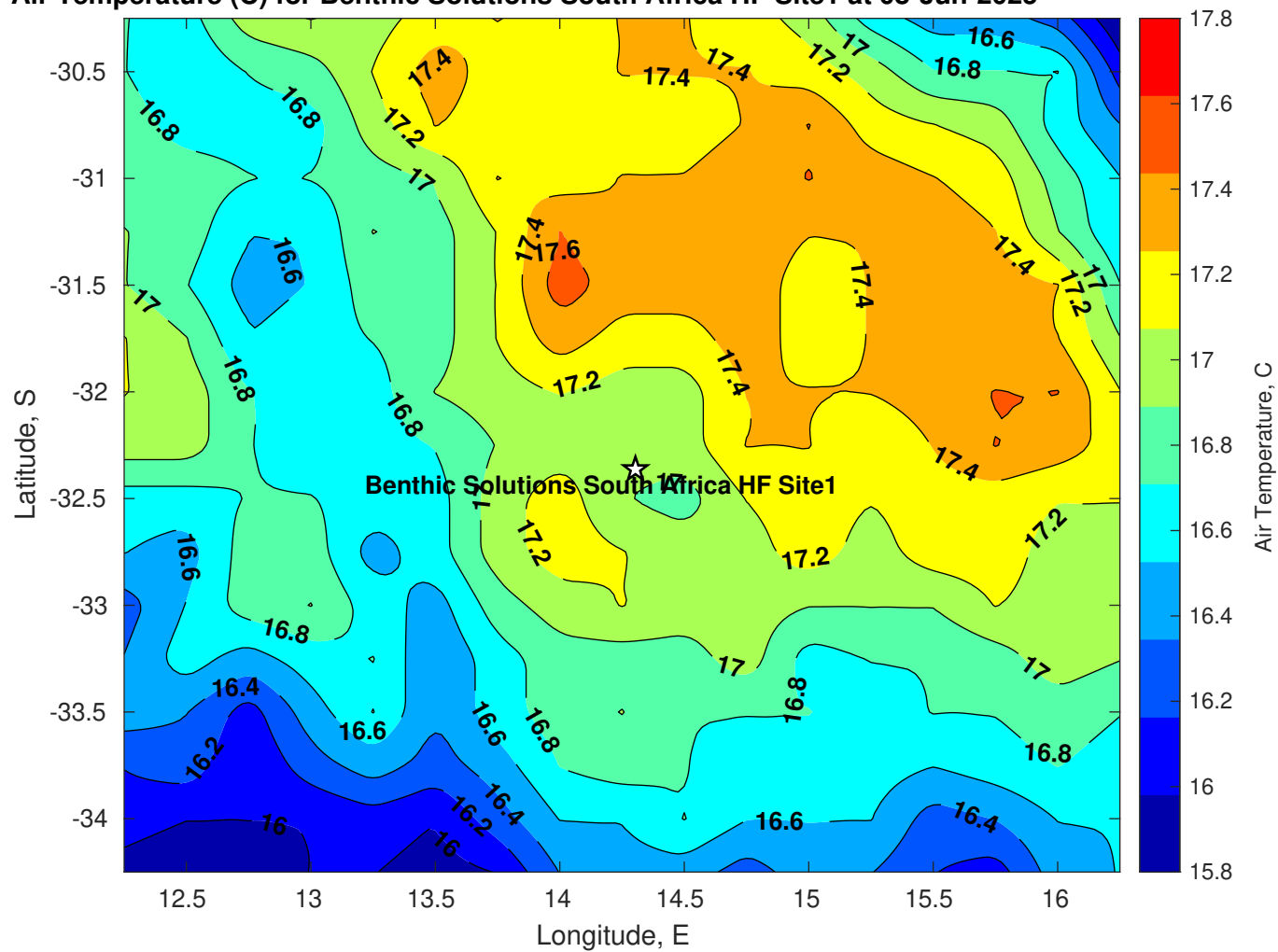
Air Temperature (C) for Benthic Solutions South Africa HF Site1 at 08-Jun-2025
