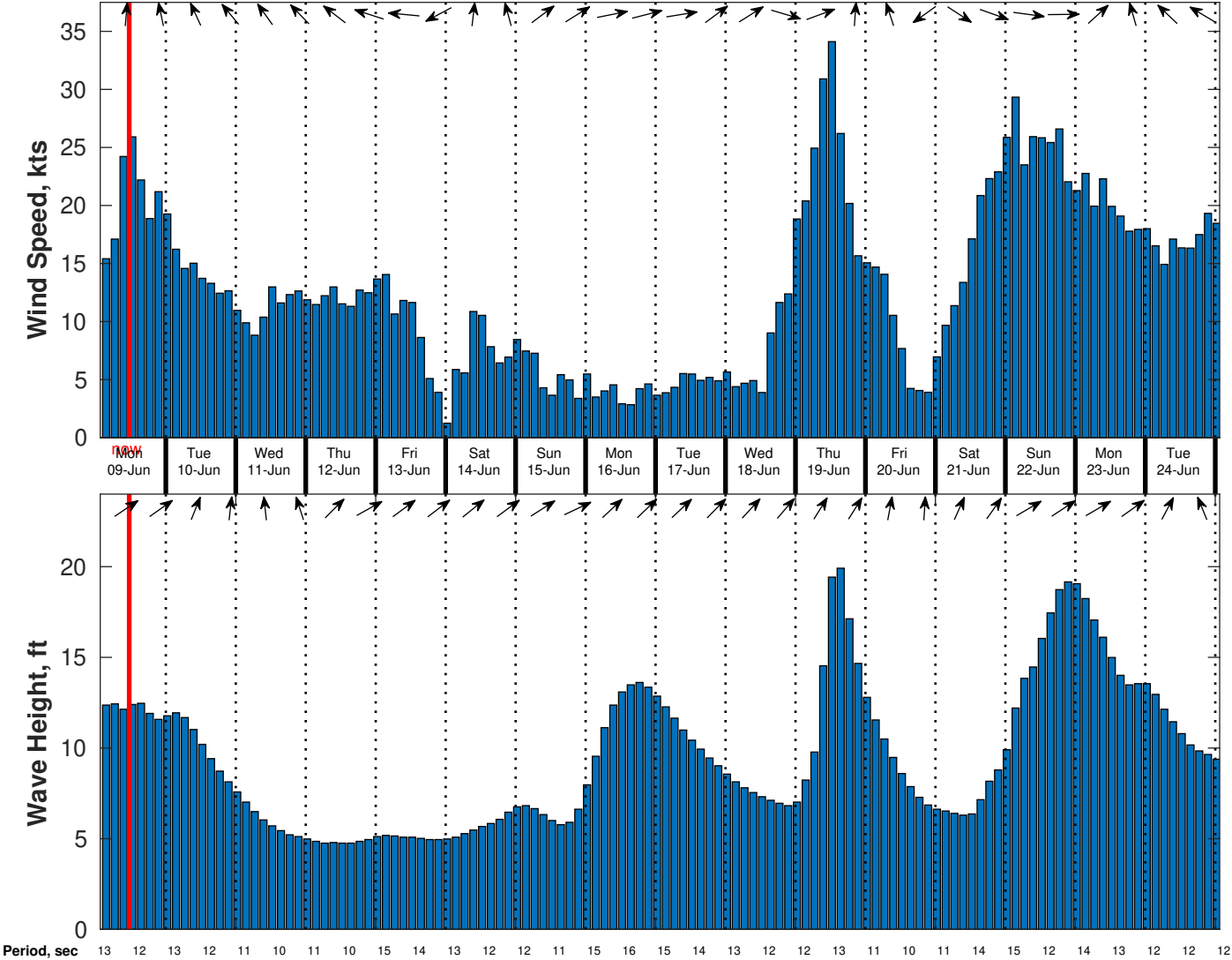
Wind & Wave Forecast for Benthic Solutions South Africa HF Site1 from 08-Jun-2025 02:00:00 to 24-Jun-2025 02:00:00
