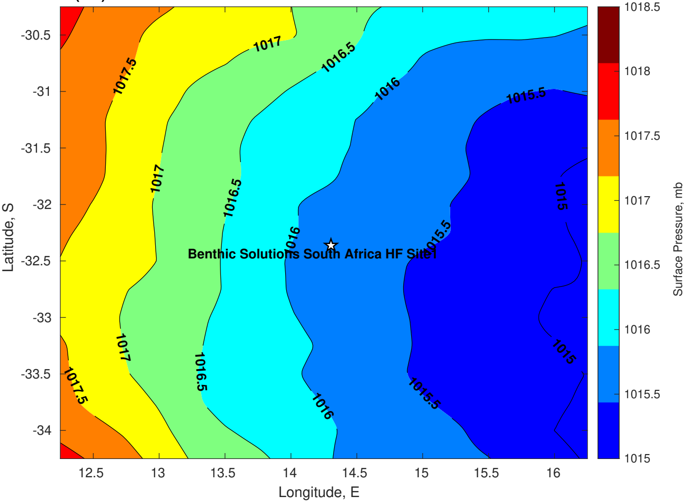
Surface Pressure (mb) for Benthic Solutions South Africa HF Site1 at 08-Jun-2025 00:00:00
