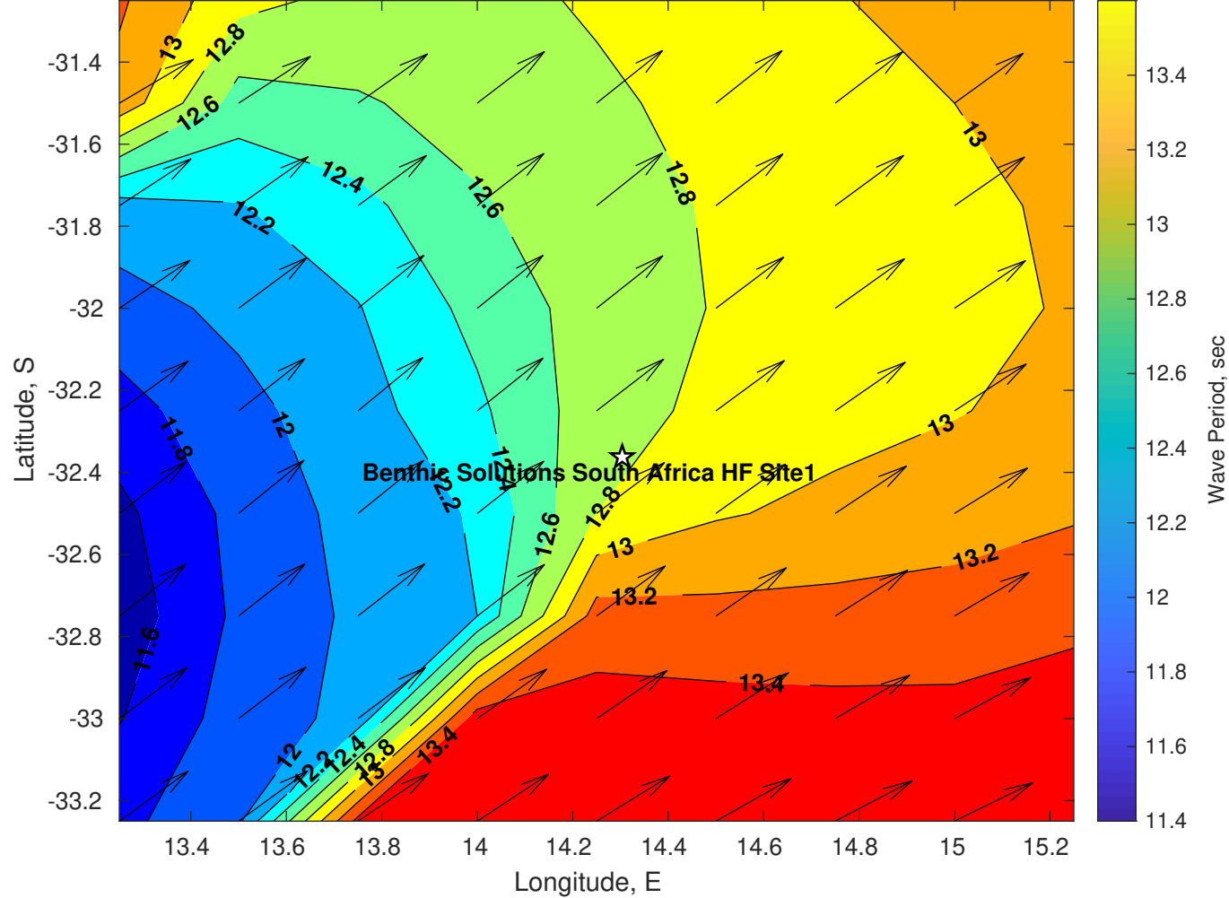
Wave Period (sec) for Benthic Solutions South Africa HF Site1 at 08-Jun-2025 09:00:00
