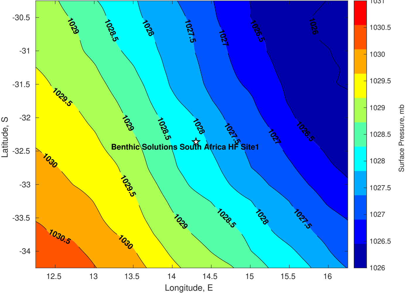
Surface Pressure (mb) for Benthic Solutions South Africa HF Site1 at 09-Jun-2025 00:00:00
