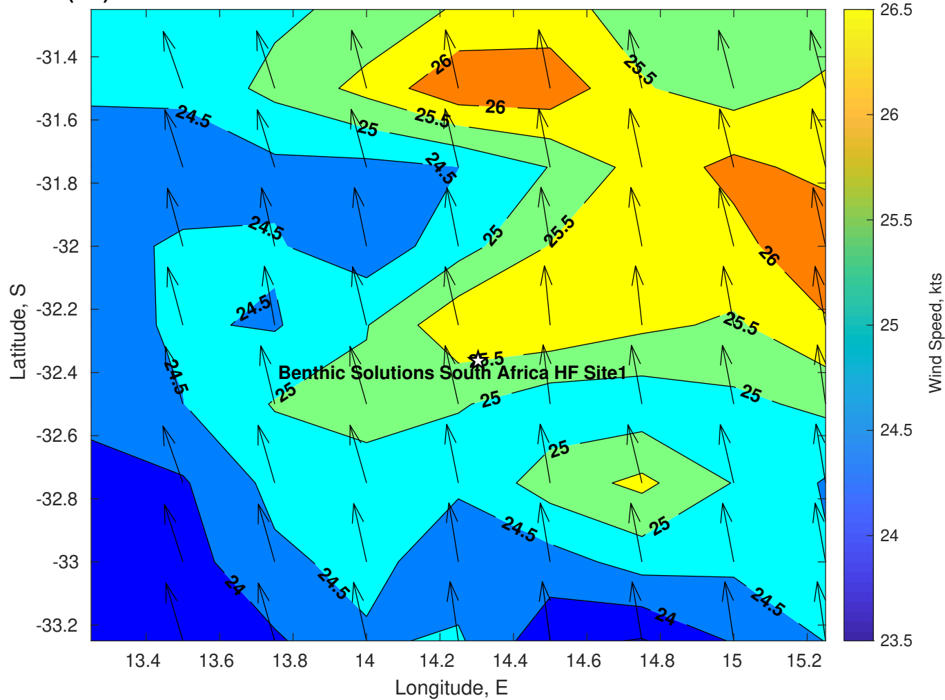
Winds (kts) for Benthic Solutions South Africa HF Site1 at 08-Jun-2025 09:00:00
