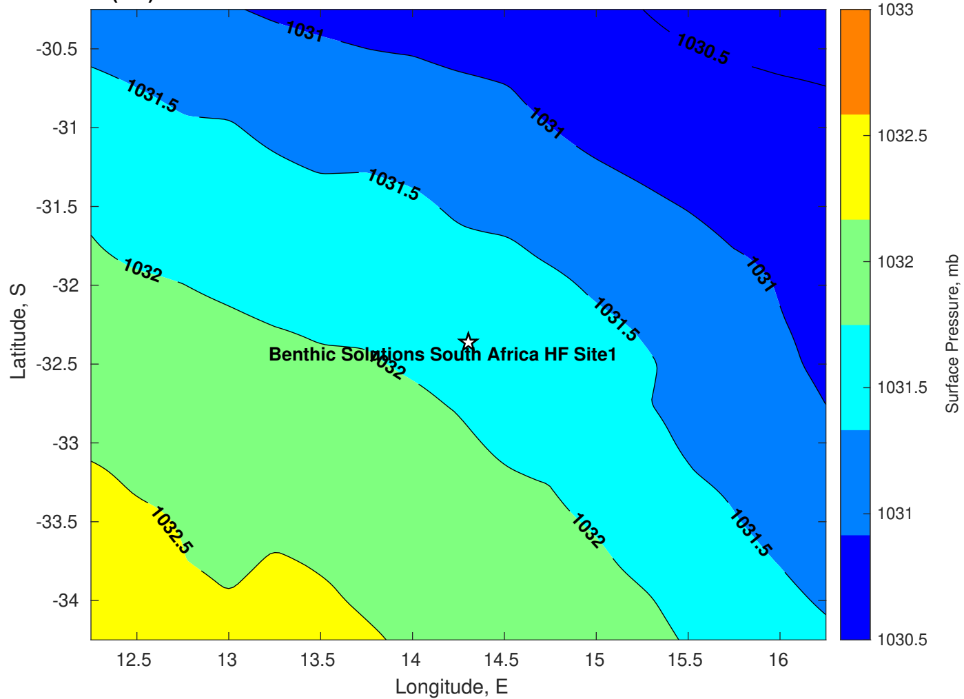
Surface Pressure (mb) for Benthic Solutions South Africa HF Site1 at 10-Jun-2025 00:00:00
