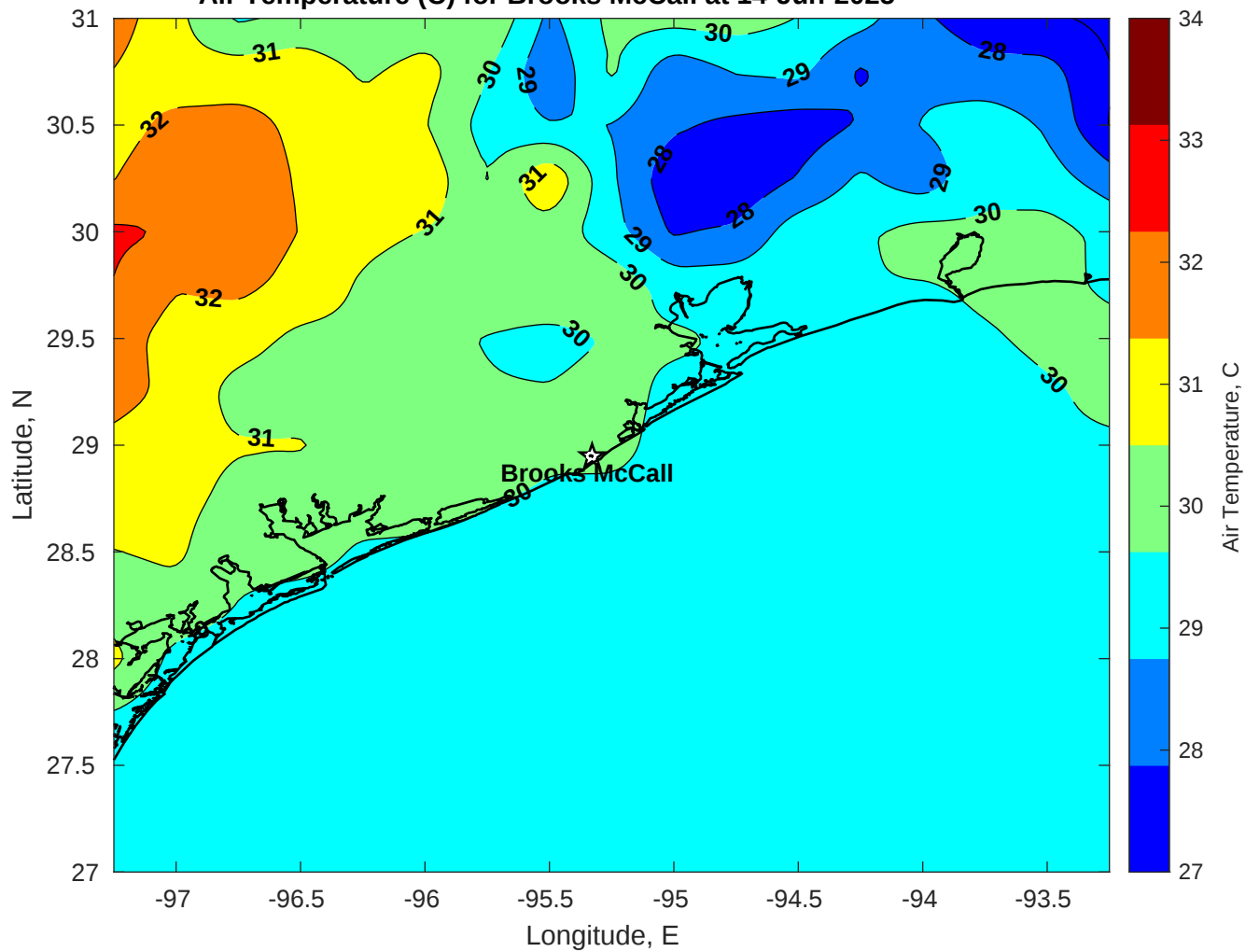
Air Temperature (C) for Brooks McCall at 14-Jun-2025
