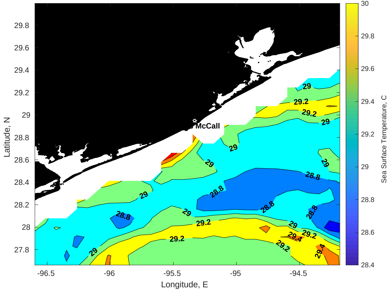
SST for Brooks McCall at 13-Jun-2025 00:00:00
