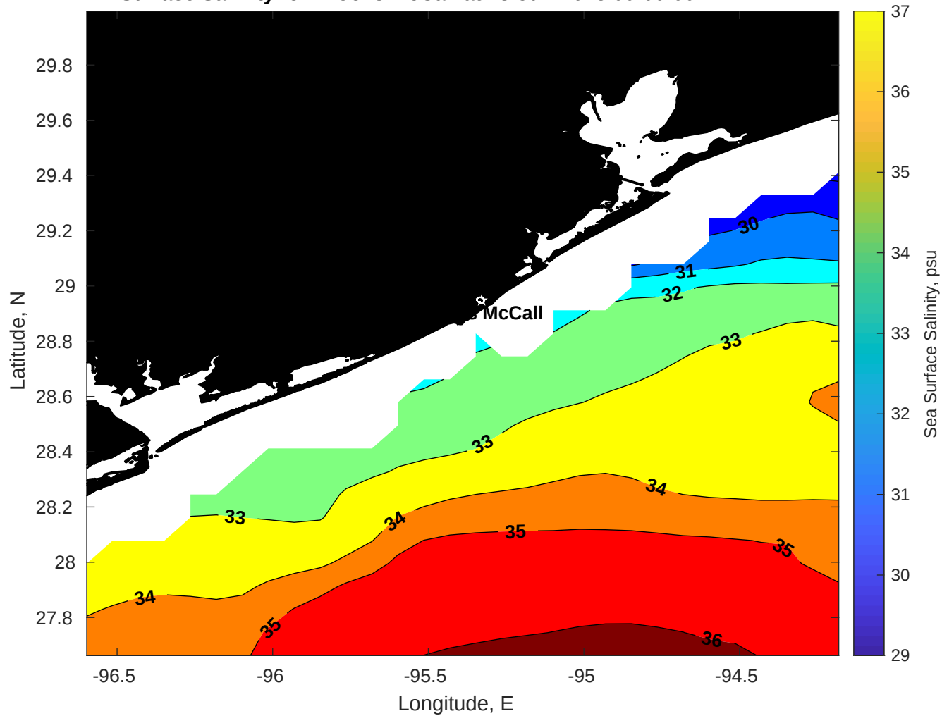
Surface Salinity for Brooks McCall at 13-Jun-2025 00:00:00
