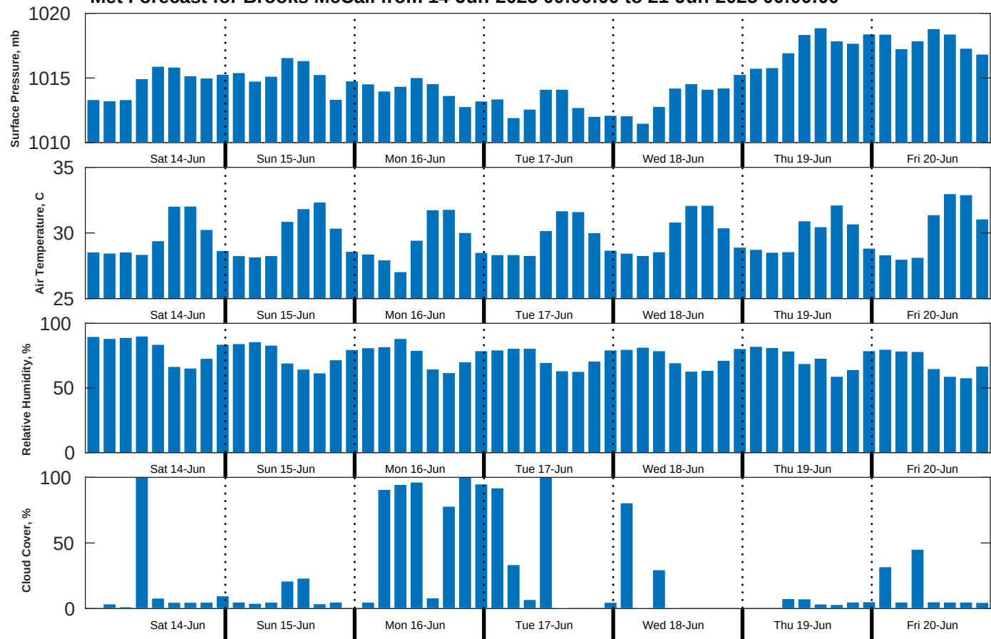
Met Forecast for Brooks McCall from 14-Jun-2025 00:00:00 to 21-Jun-2025 00:00:00
