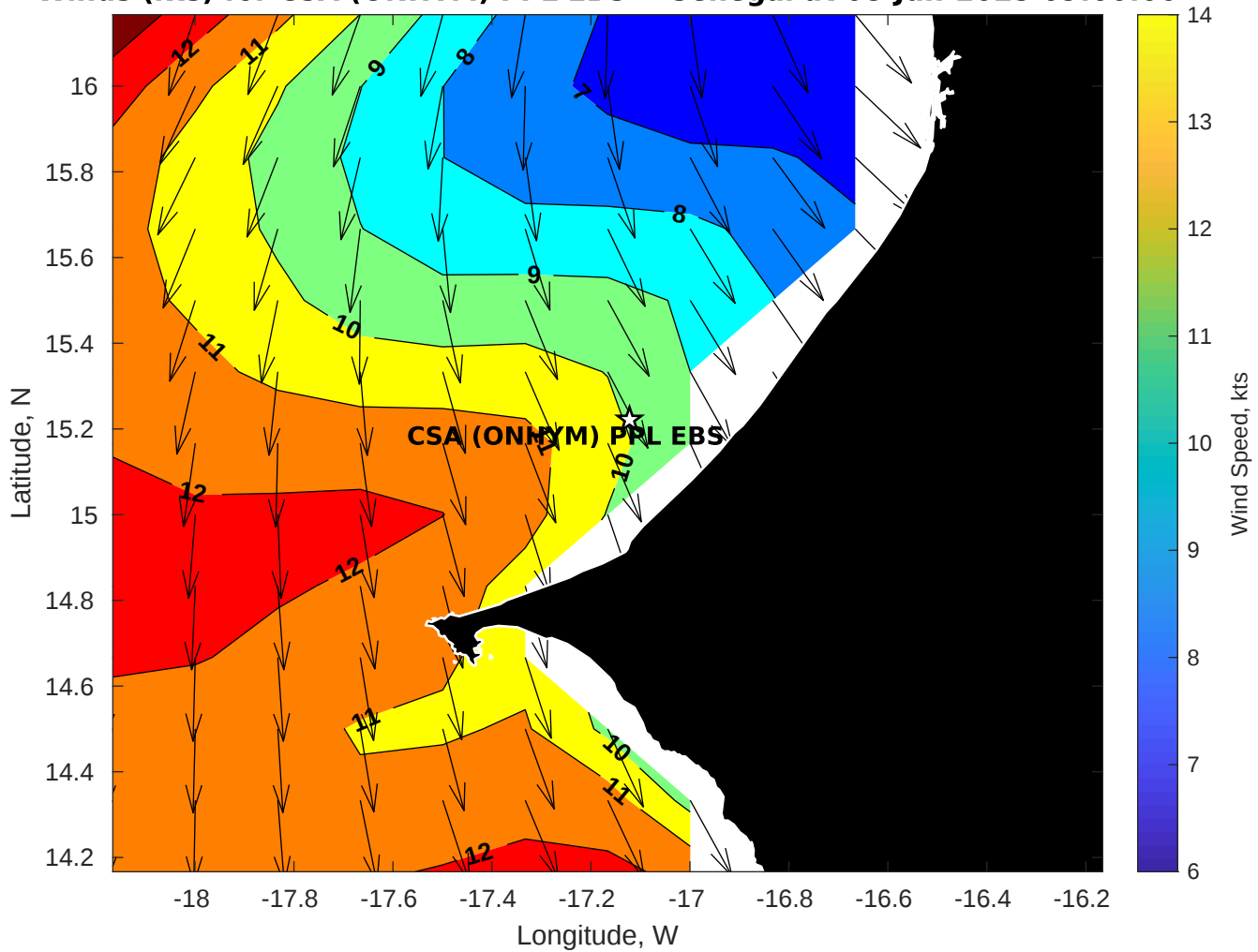
Winds (kts) for CSA (ONHYM) PPL EBS - Senegal at 08-Jun-2025 09:00:00
