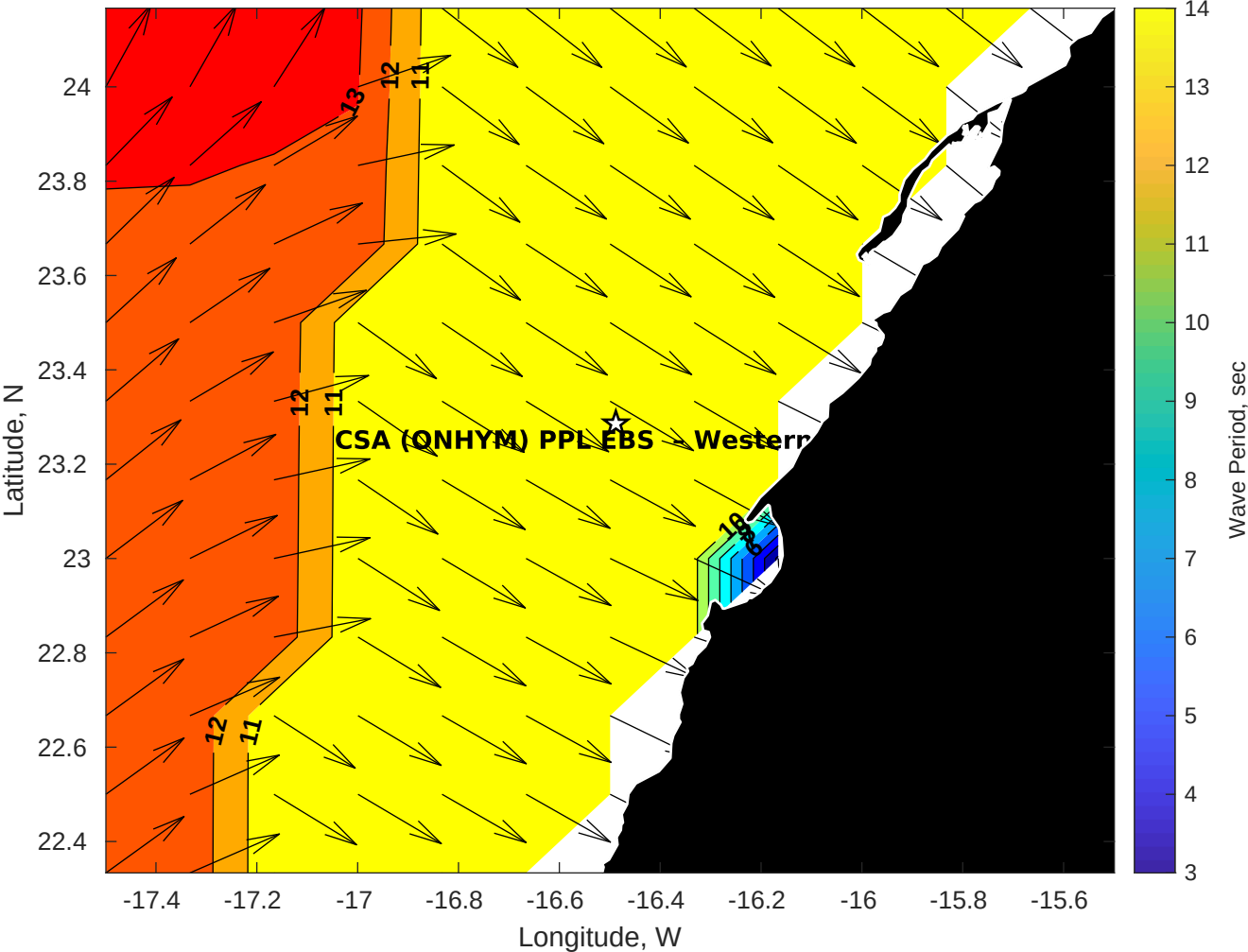
Wave Period (sec) for CSA (ONHYM) PPL EBS - Western Sahara at 08-Jun-2025 09:00:00
