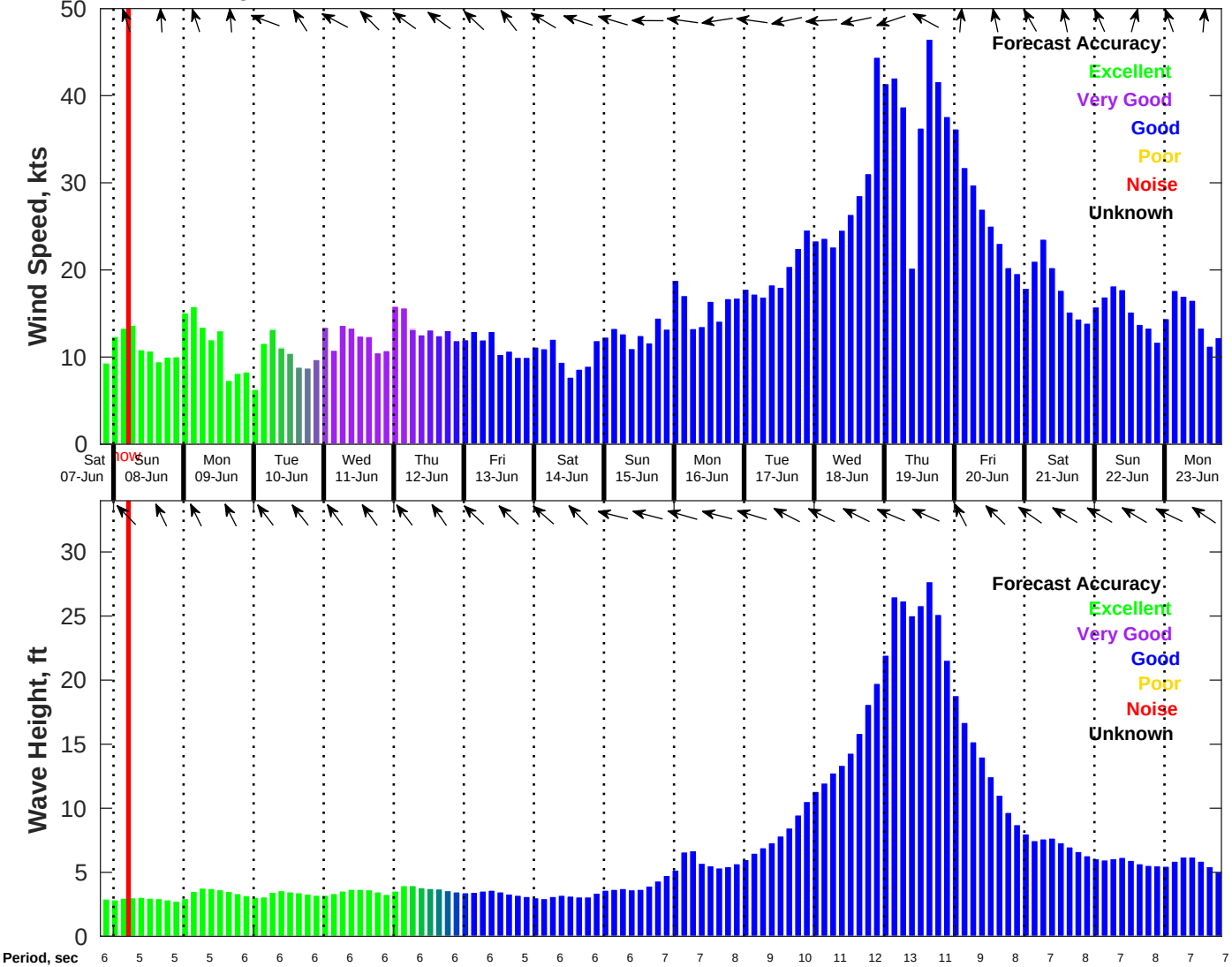
Wind & Wave Forecast for CTI Enbridge Kaskida & Tiber PPL Geotechnical from 07-Jun-2025 20:00:00 to 23-Jun-2025 20:00:00
