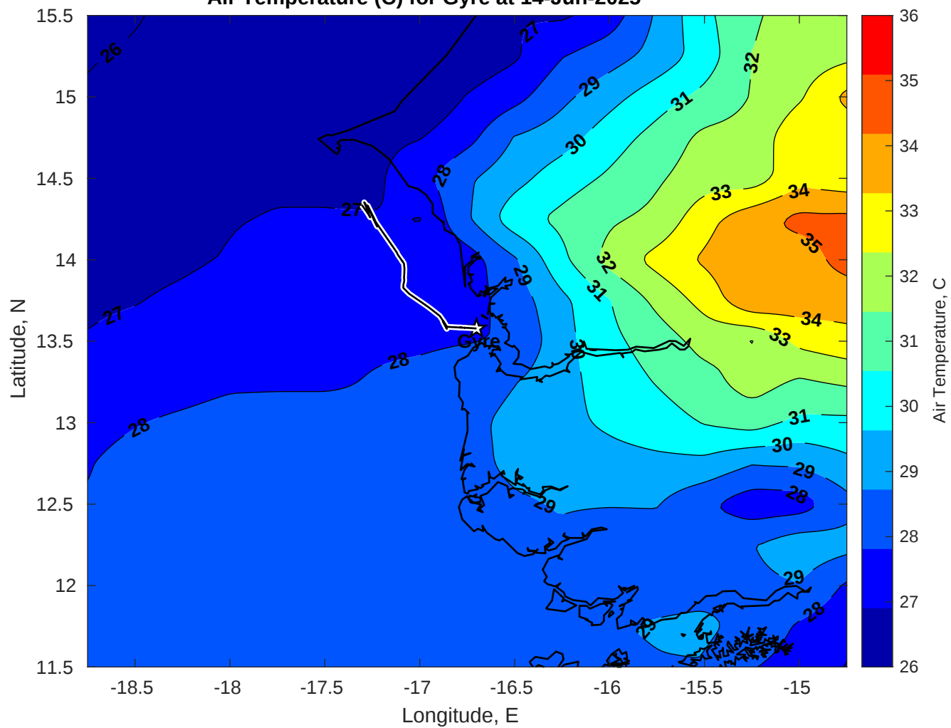
Air Temperature (C) for Gyre at 14-Jun-2025
