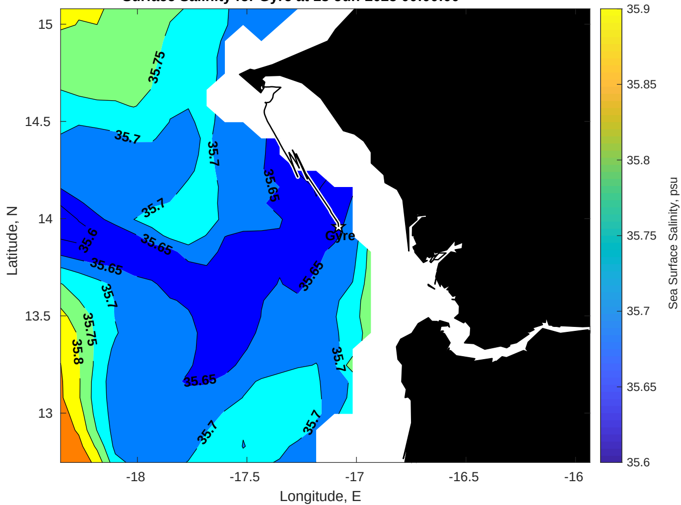
Surface Salinity for Gyre at 13-Jun-2025 00:00:00
