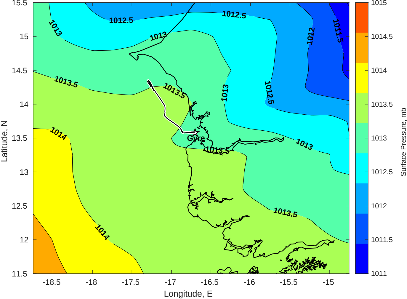
Surface Pressure (mb) for Gyre at 16-Jun-2025 00:00:00
