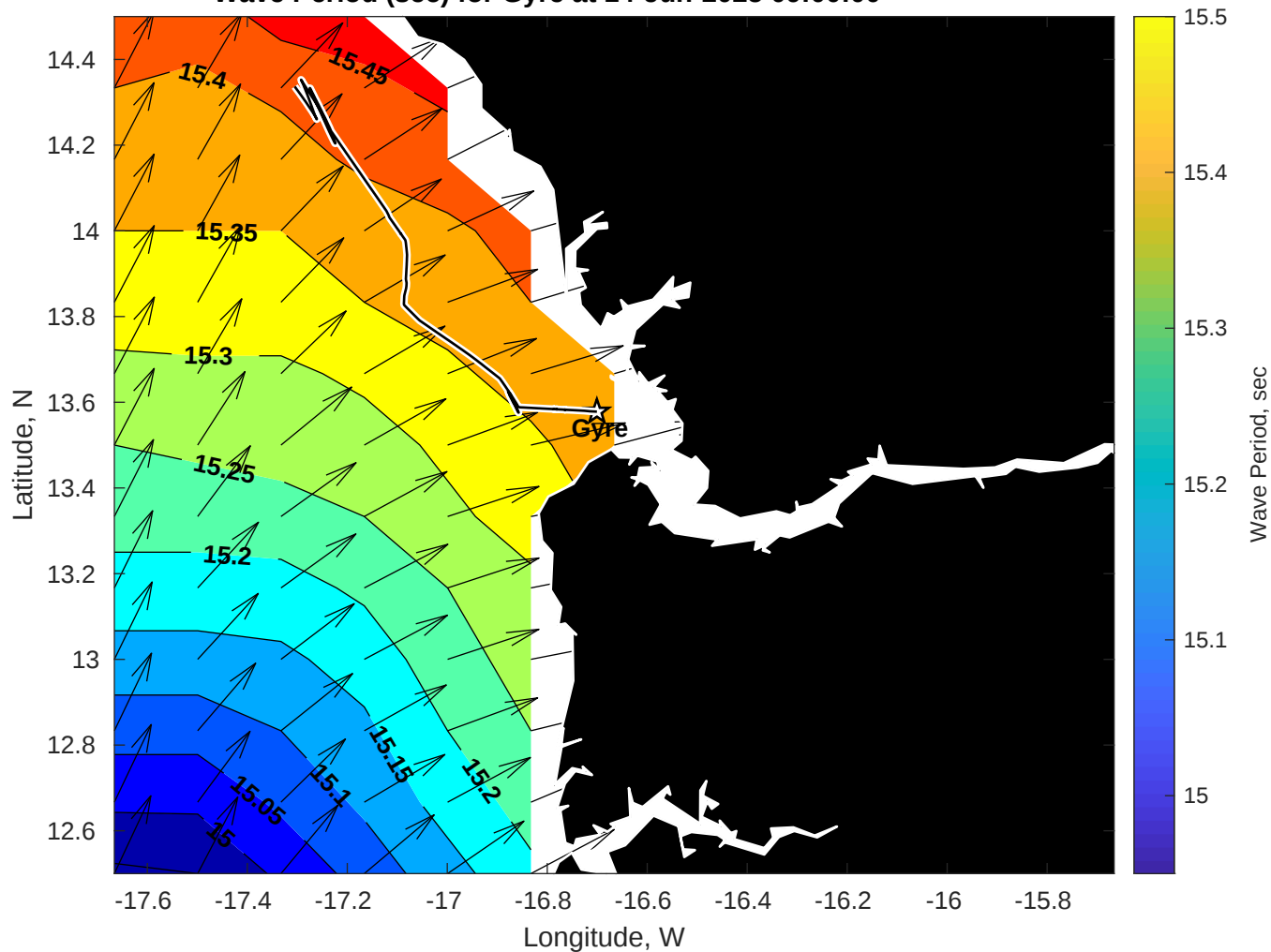
Wave Period (sec) for Gyre at 14-Jun-2025 09:00:00
