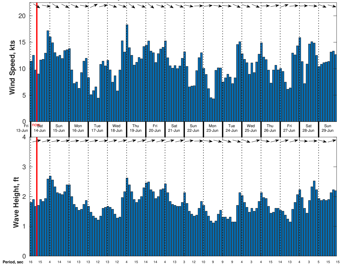
Wind & Wave Forecast for Gyre from 13-Jun-2025 23:00:00 to 29-Jun-2025 23:00:00
