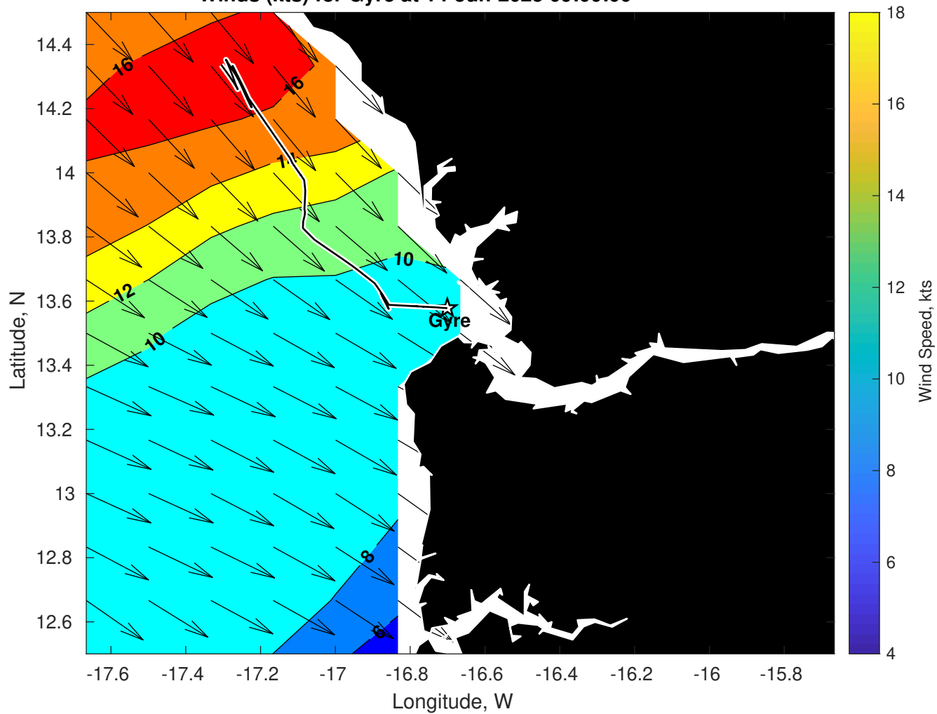
Winds (kts) for Gyre at 14-Jun-2025 09:00:00
