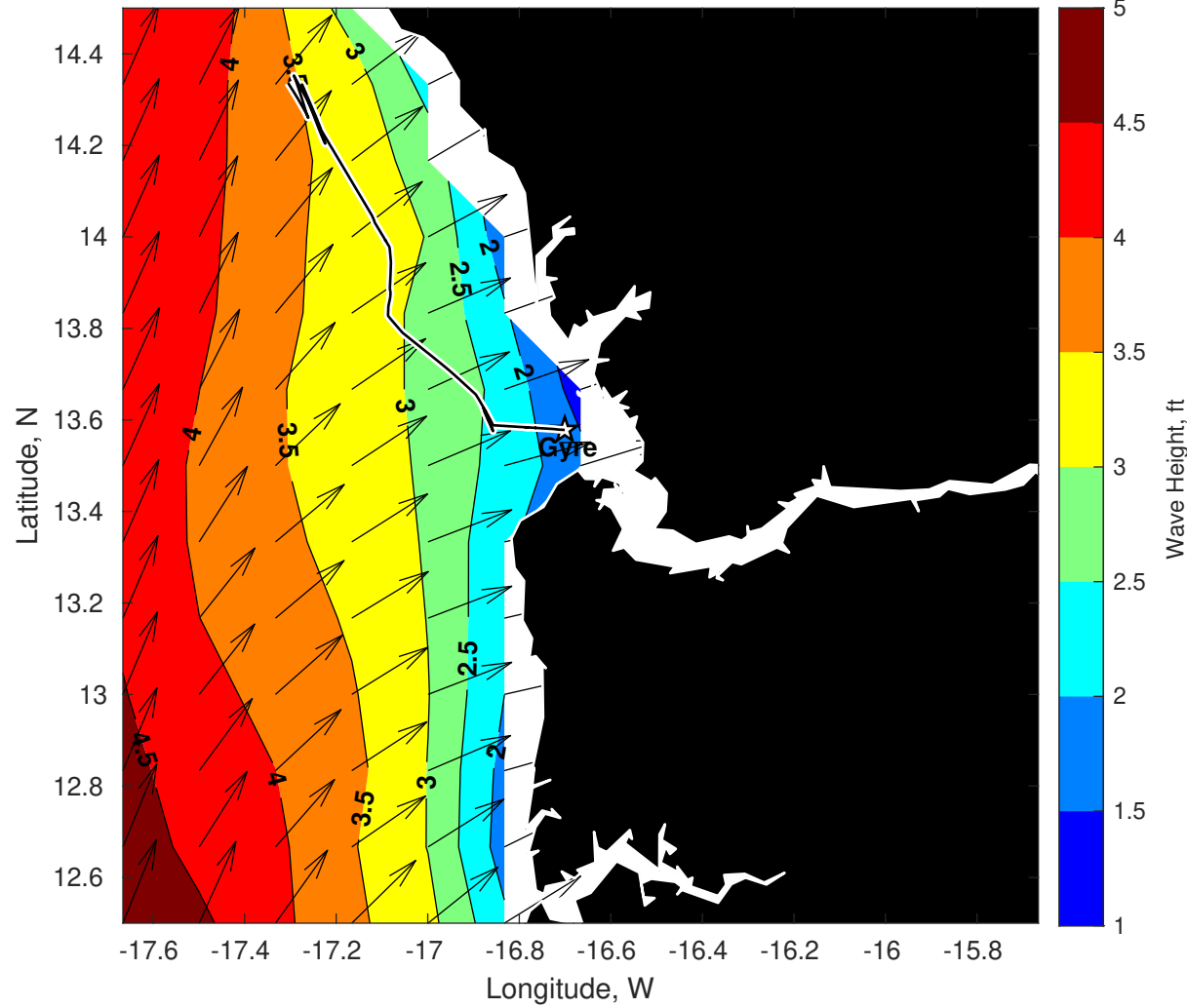
Wave Height (ft) for Gyre at 14-Jun-2025 09:00:00
