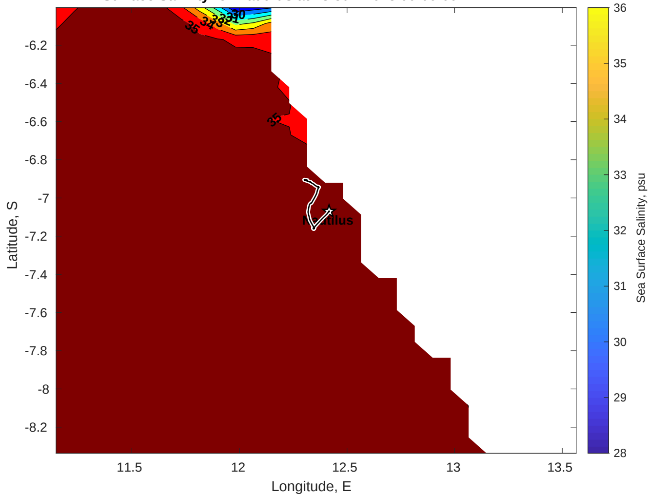
Surface Salinity for Nautilus at 13-Jun-2025 00:00:00
