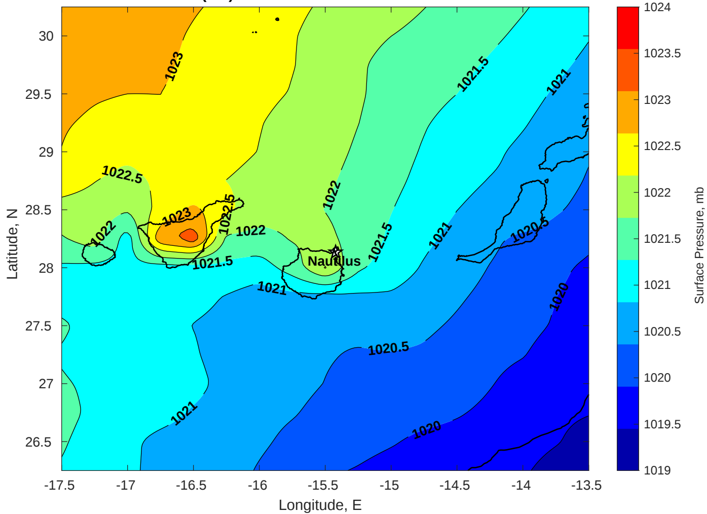
Surface Pressure (mb) for Nautilus at 14-Jun-2025 00:00:00
