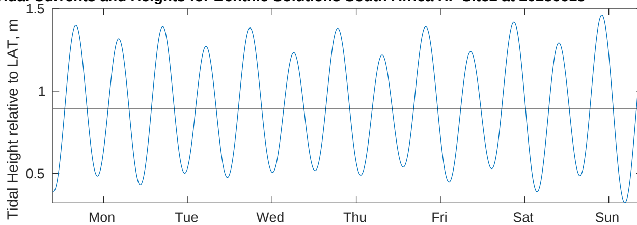
Tidal Currents and Heights for Benthic Solutions South Africa HF Site2 at 20250615
