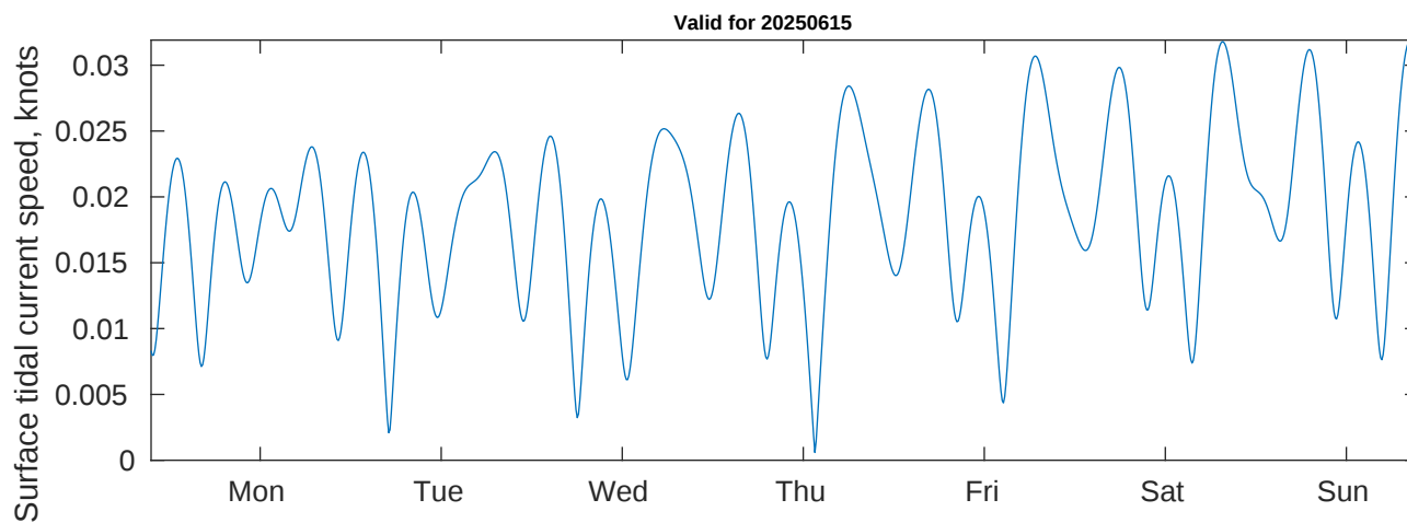
Tidal Currents and Heights for Benthic Solutions South Africa HF Site2 at 20250615
