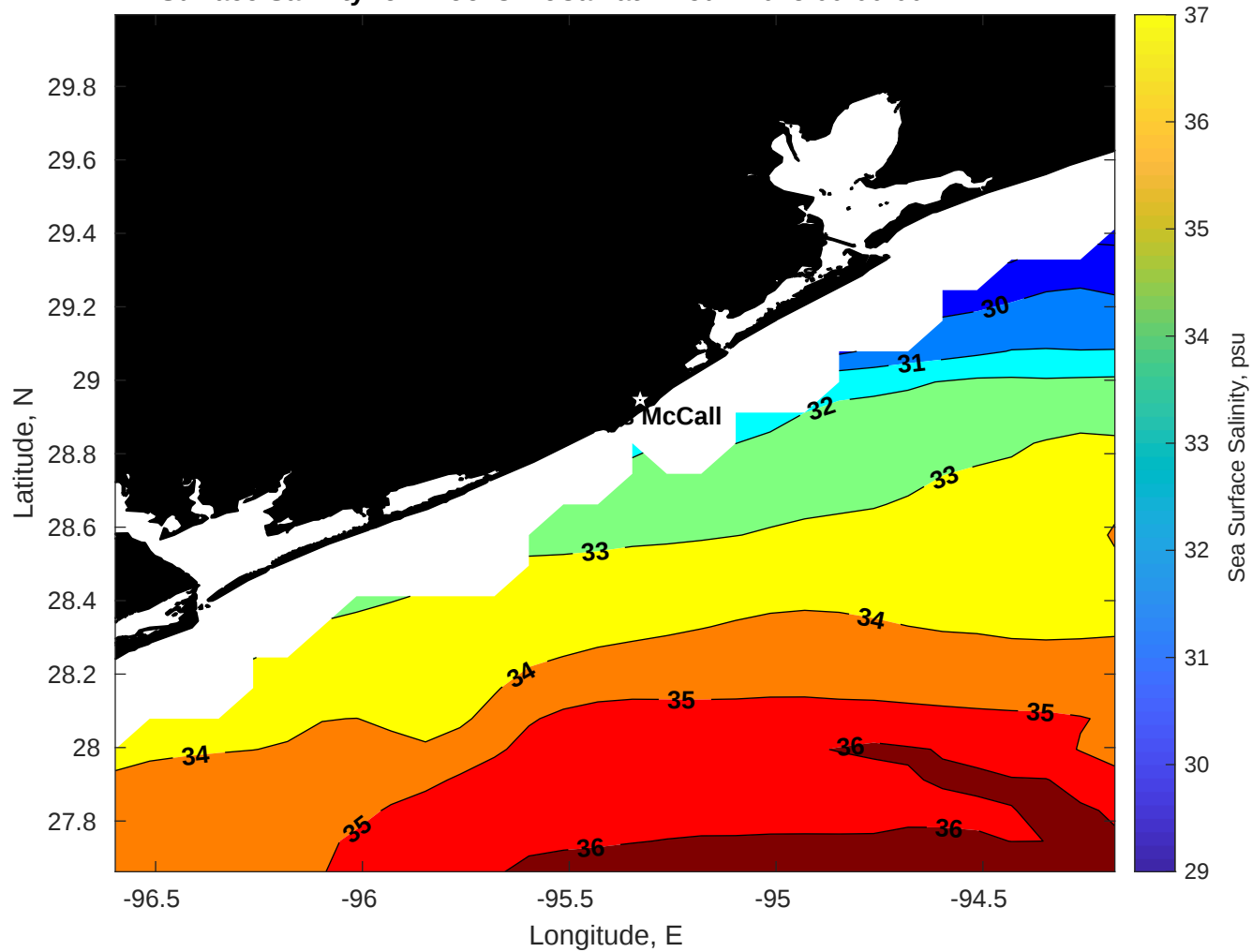
Surface Salinity for Brooks McCall at 14-Jun-2025 00:00:00
