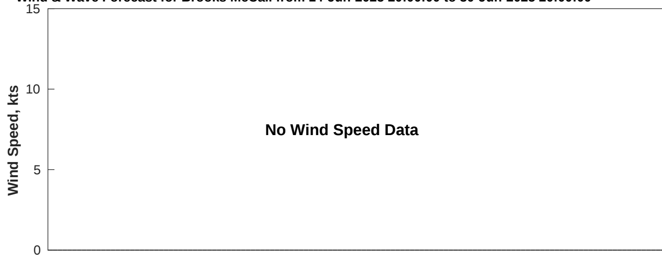
Wind & Wave Forecast for Brooks McCall from 14-Jun-2025 20:00:00 to 30-Jun-2025 20:00:00
