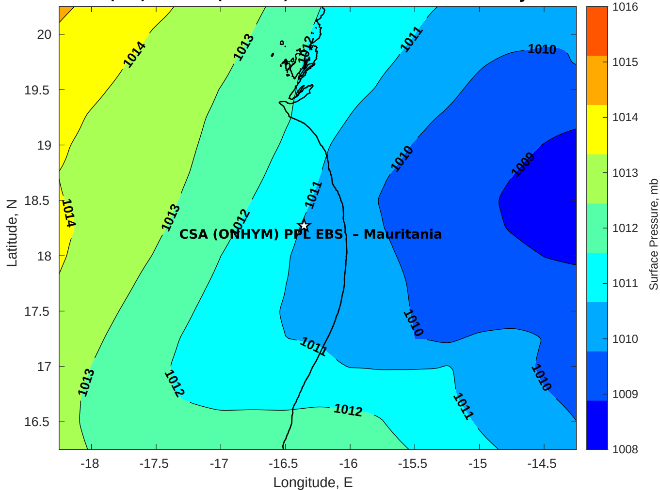
Surface Pressure (mb) for CSA (ONHYM) PPL EBS - Mauritania at 16-Jun-2025 00:00:00
