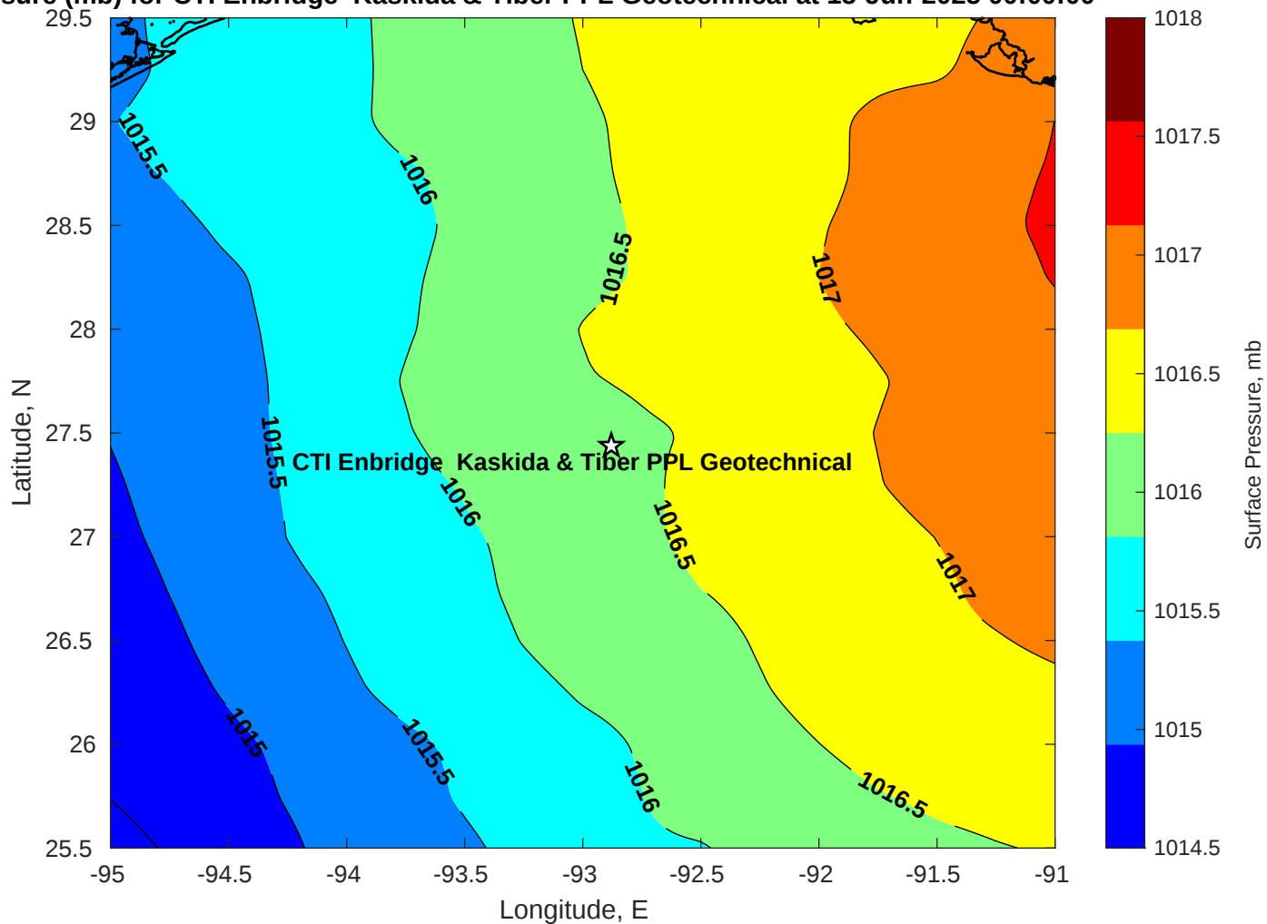
Surface Pressure (mb) for CTI Enbridge Kaskida & Tiber PPL Geotechnical at 15-Jun-2025 00:00:00
