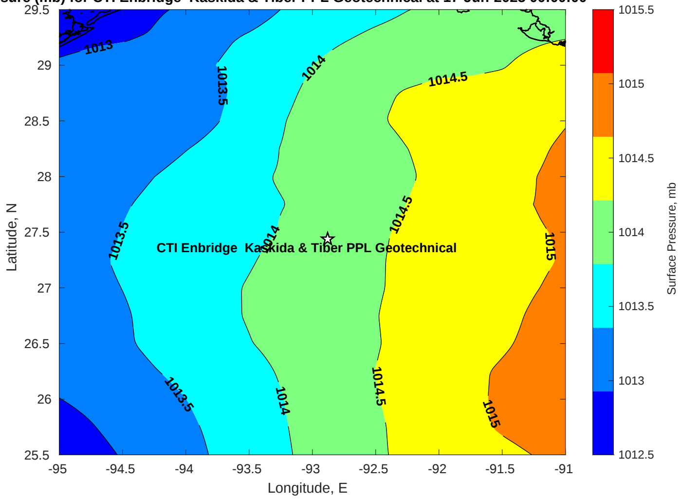
Surface Pressure (mb) for CTI Enbridge Kaskida & Tiber PPL Geotechnical at 17-Jun-2025 00:00:00
