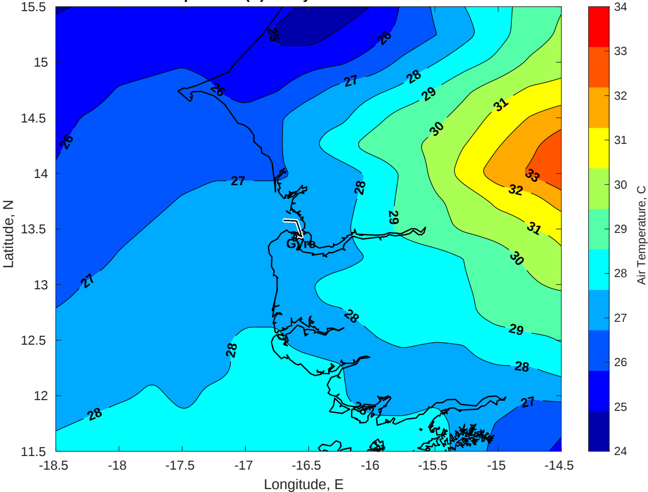
Air Temperature (C) for Gyre at 15-Jun-2025
