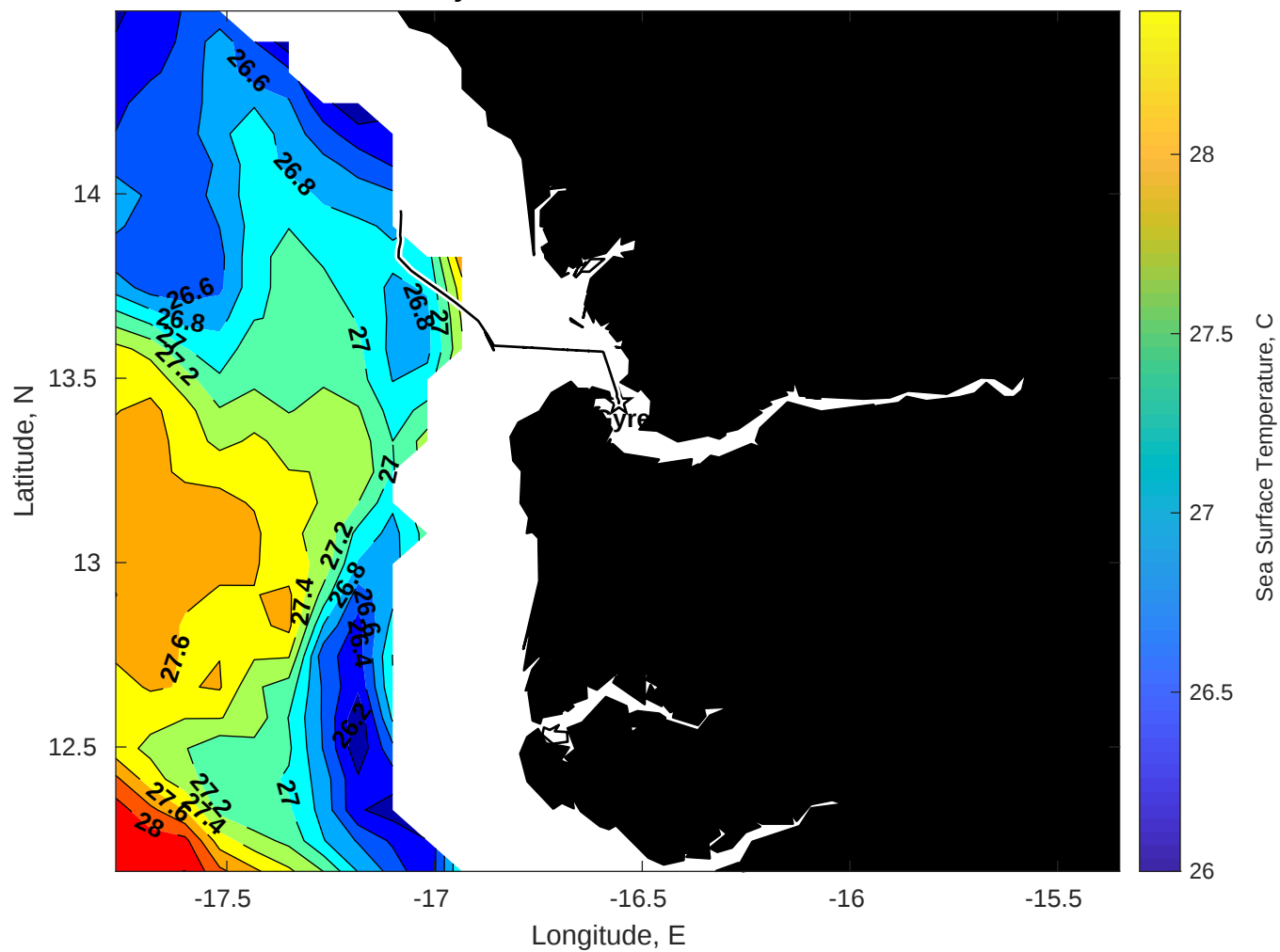
SST for Gyre at 14-Jun-2025 00:00:00
