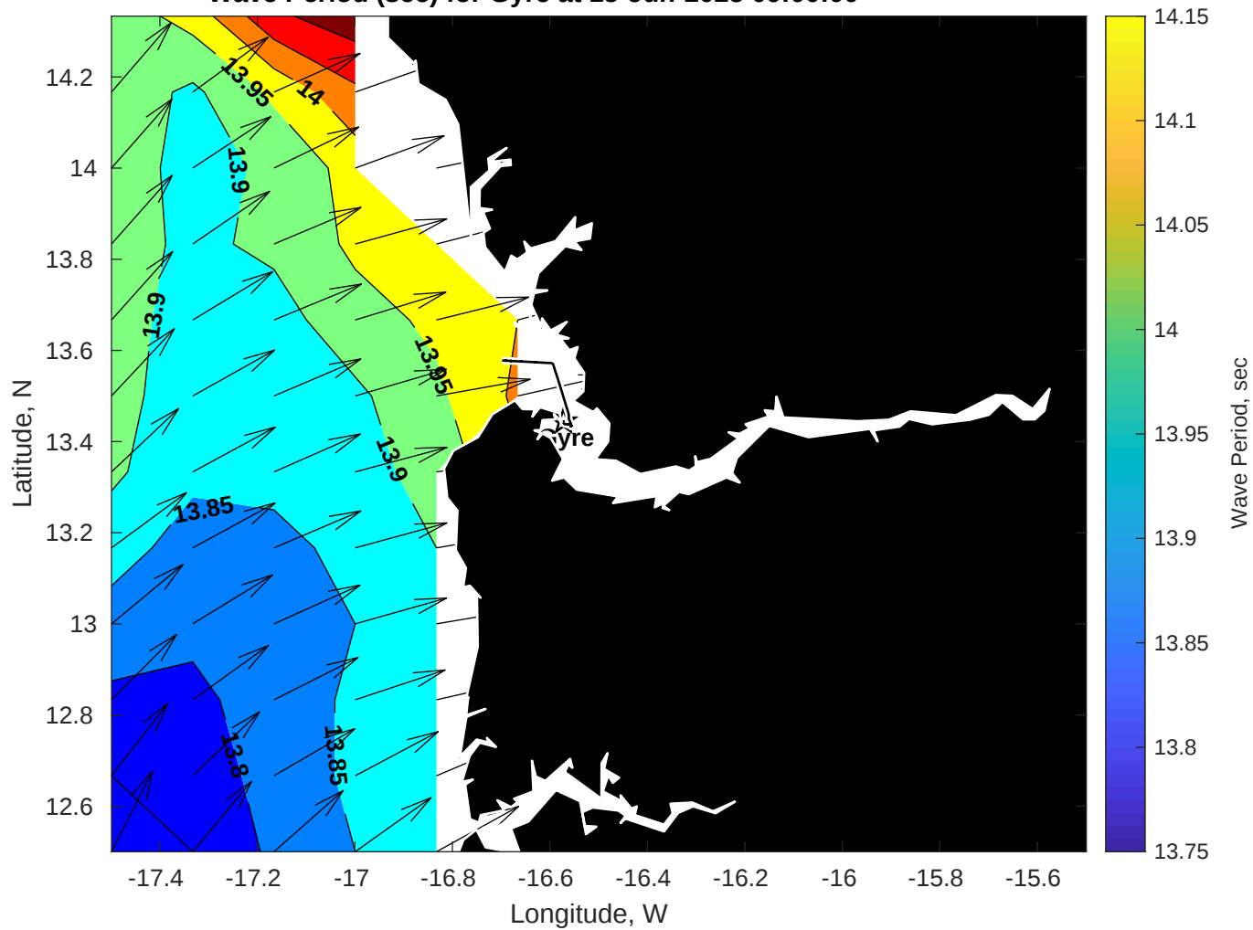
Wave Period (sec) for Gyre at 15-Jun-2025 09:00:00
