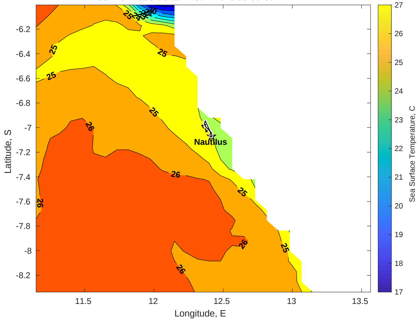
SST for Nautilus at 14-Jun-2025 00:00:00
