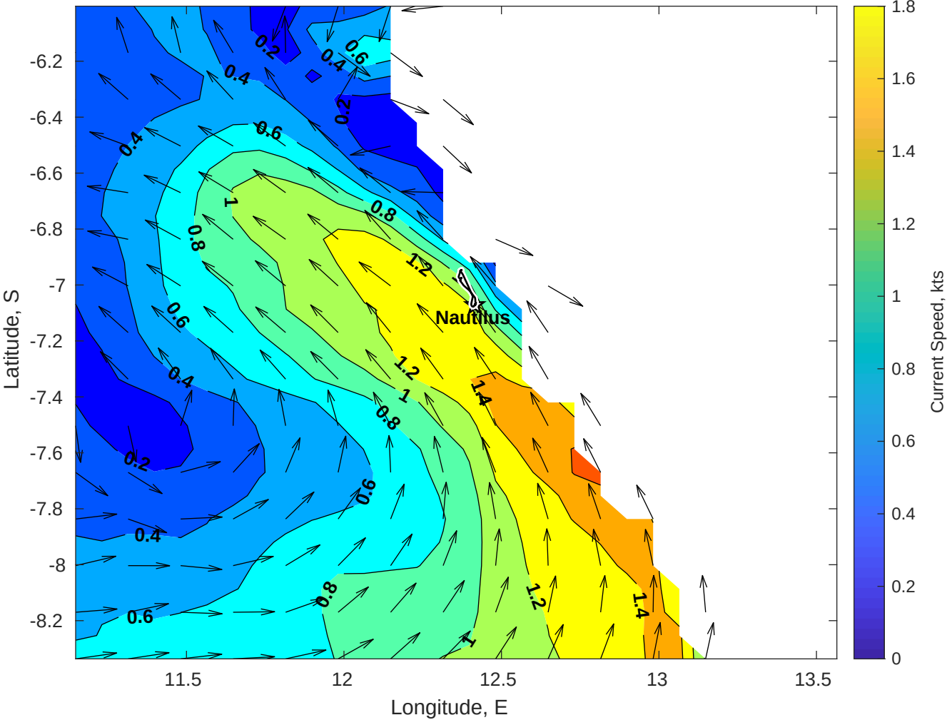
Surface Currents for Nautilus at 14-Jun-2025 00:00:00
