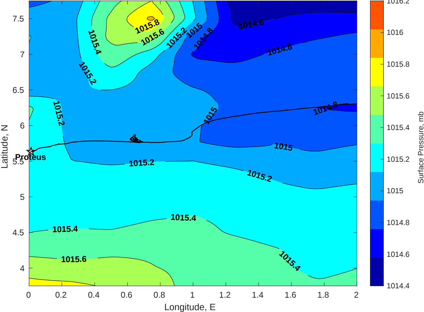
Surface Pressure (mb) for Proteus at 16-Jun-2025 00:00:00
