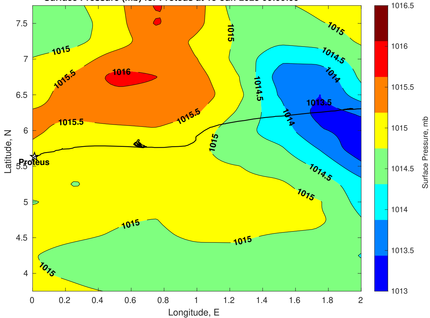
Surface Pressure (mb) for Proteus at 15-Jun-2025 00:00:00
