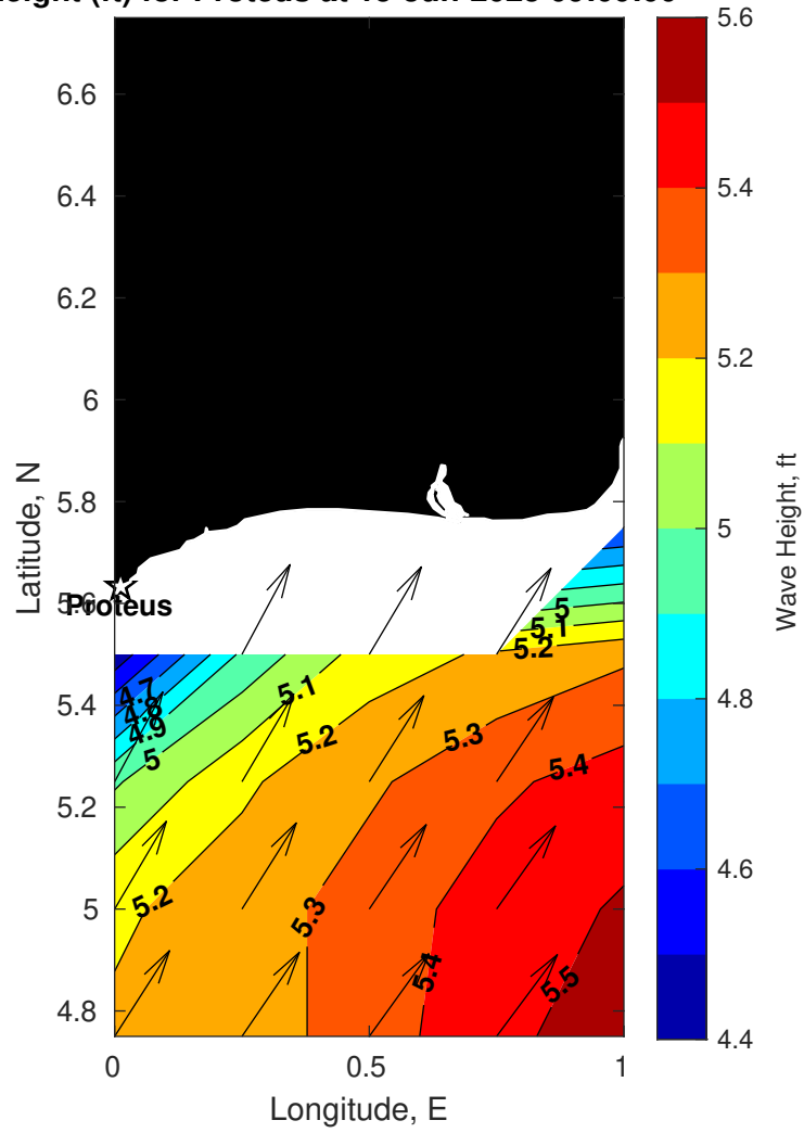
Wave Height (ft) for Proteus at 15-Jun-2025 09:00:00
