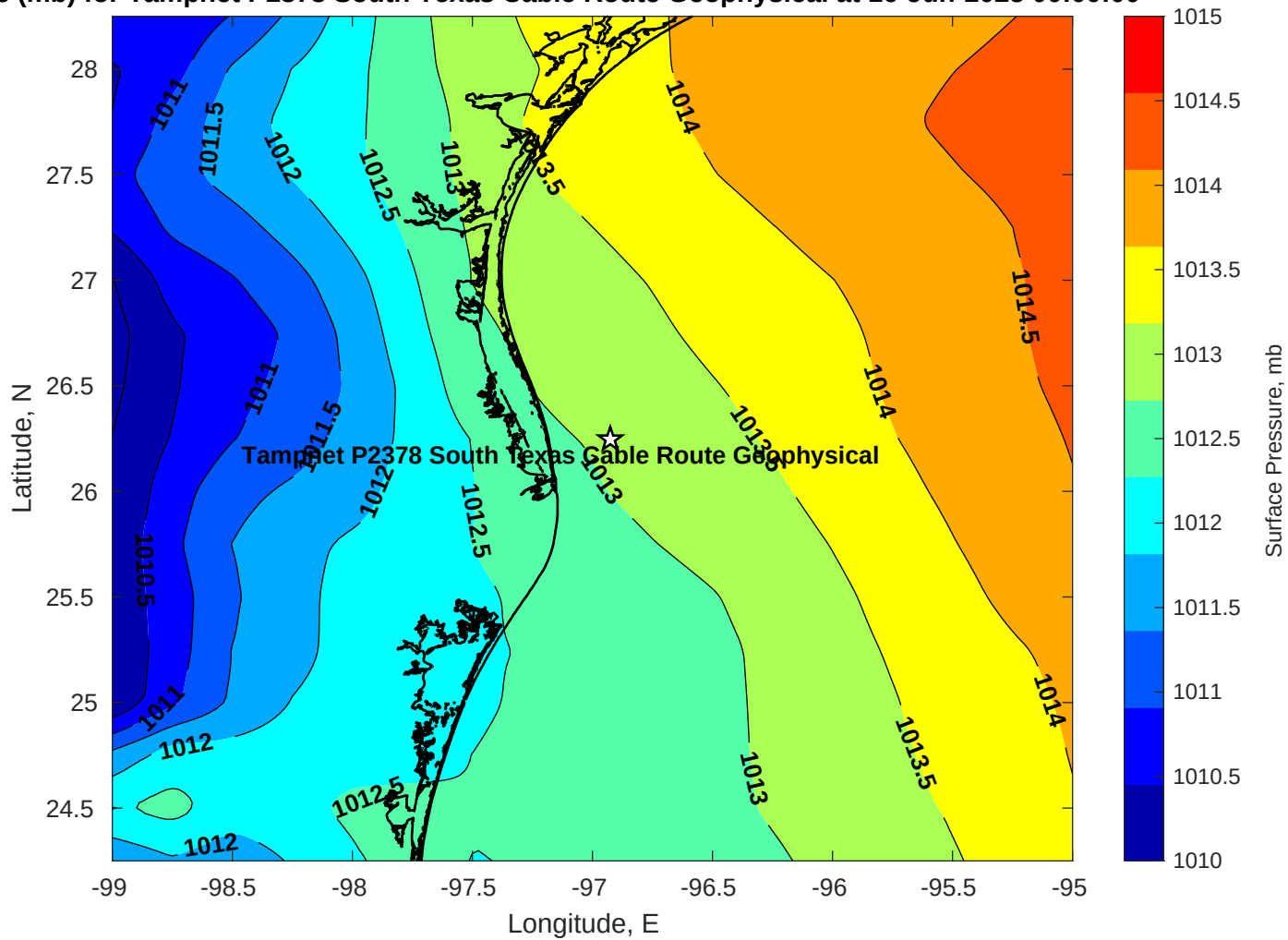
Pressure (mb) for Tampnet P2378 South Texas Cable Route Geophysical at 16-Jun-2025 00:00:00
